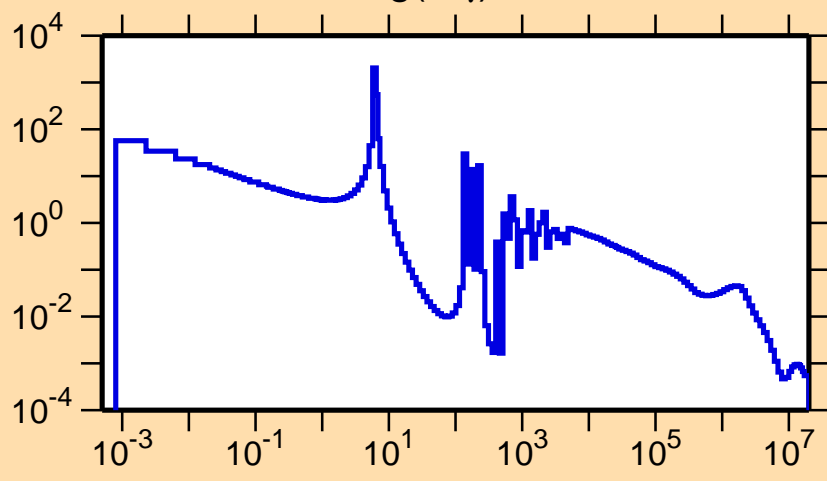
\sigma vs. E for ^{117}\text{Ag}(n,\gamma)
