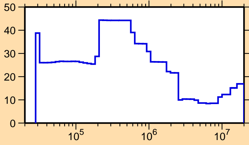
\Delta\sigma/\sigma vs. E for ^{117}\text{Ag}(n,\text{nonel.})
