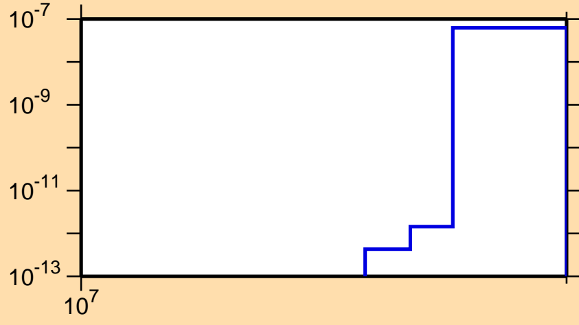
\sigma vs. E for ^{117}\text{Ag}(n,\text{nd})
