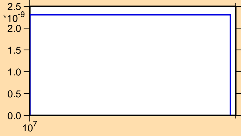
\sigma vs. E for ^{117}\text{Ag}(n,nt)
