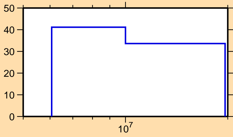
\Delta\sigma/\sigma vs. E for ^{117}\text{Ag}(n,el.)
