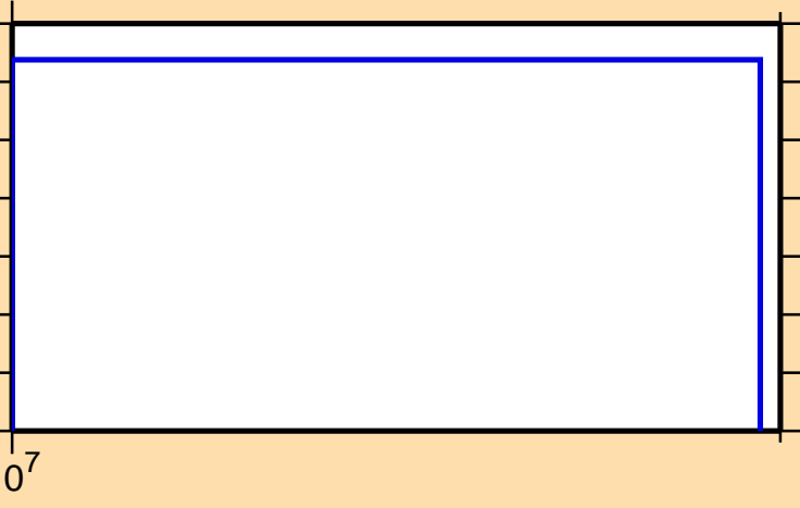
\sigma vs. E for ^{117}\text{Ag}(n,np)
