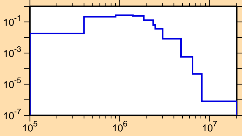
\sigma vs. E for ^{117}\text{Ag}(n,n_3)
