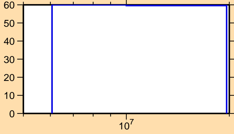
\Delta\sigma/\sigma vs. E for ^{118}\text{Ag}(n,p)
