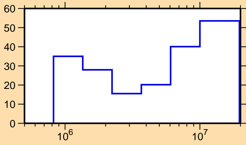
\Delta\sigma/\sigma vs. E for ^{118}\text{Ag}(n,n\text{cont.})
