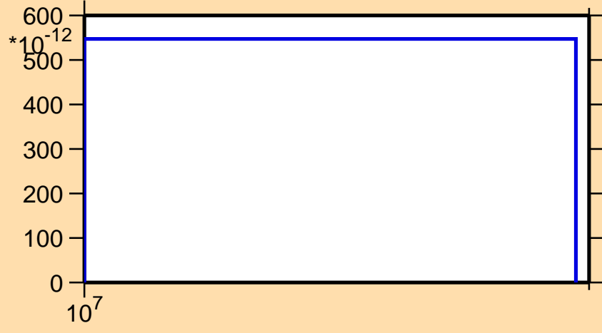
\sigma vs. E for ^{118}\text{Ag}(n,2np)
