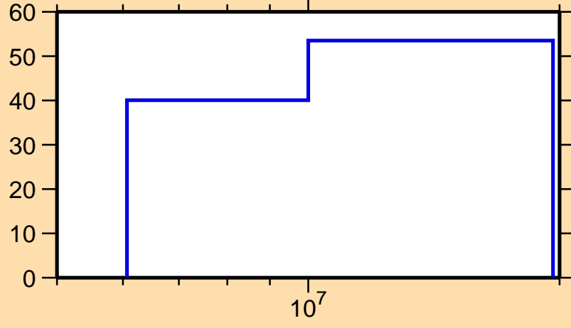
\Delta\sigma/\sigma vs. E for ^{118}\text{Ag}(n,n\text{cont.})
