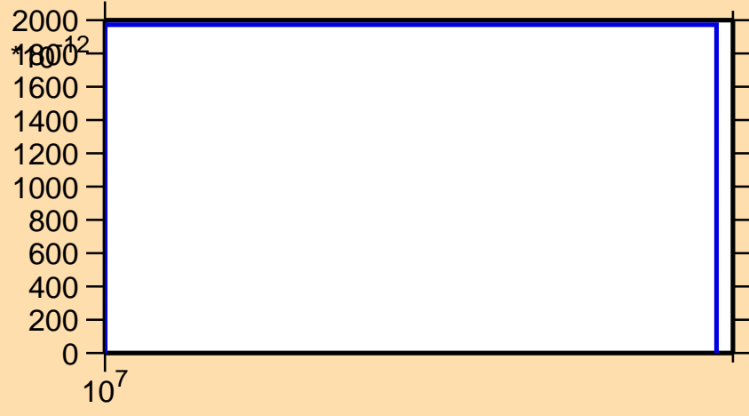
\sigma vs. E for ^{118}\text{Ag}(n,nt)
