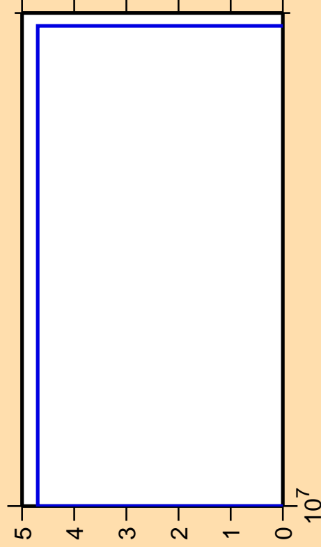
\Delta\sigma/\sigma vs. E for ^{118}\text{Ag}(n,2n\alpha)
