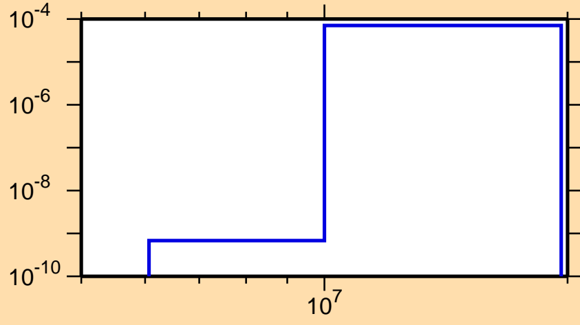
\sigma vs. E for ^{118}\text{Ag}(n,\alpha)
