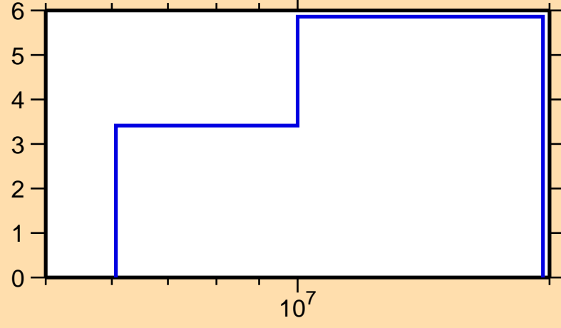
\Delta\sigma/\sigma vs. E for ^{118}\text{Ag}(n,\text{tot.})
