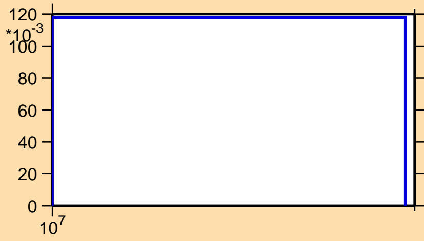
\sigma vs. E for ^{118}\text{Ag}(n,3n)
