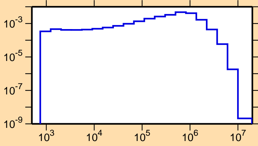
\sigma vs. E for ^{118}\text{Ag}(n,n_2)
