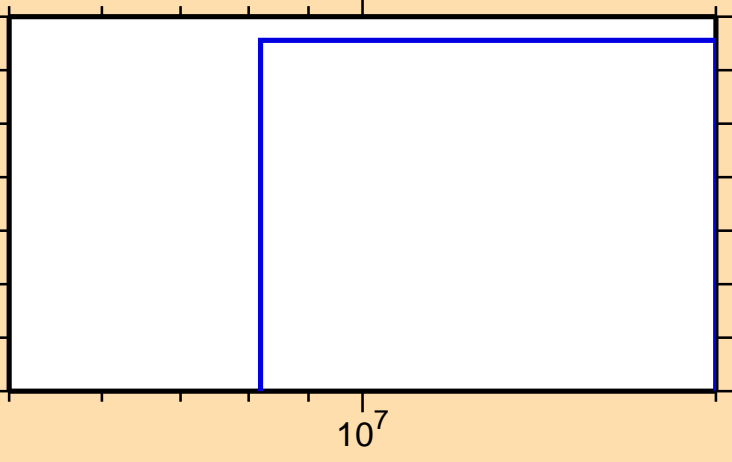
\sigma vs. E for ^{119}\text{Ag}(n,t)
