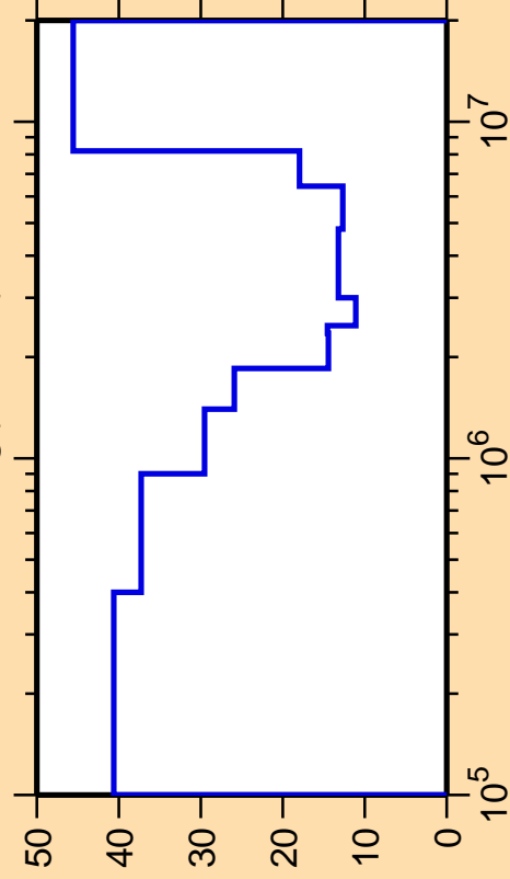
\Delta\sigma/\sigma vs. E for ^{119}\text{Ag}(n,\text{inel.})
