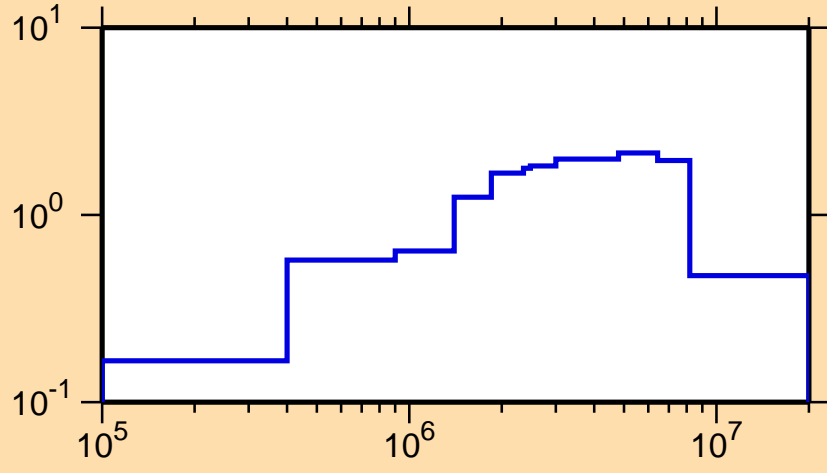
\sigma vs. E for ^{119}\text{Ag}(n,\text{inel.})
