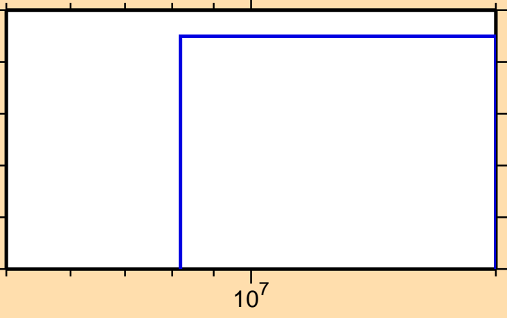
\sigma vs. E for ^{119}\text{Ag}(n,n\alpha)
