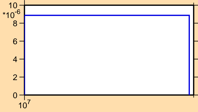
\sigma vs. E for ^{120}\text{Ag}(n,np)
