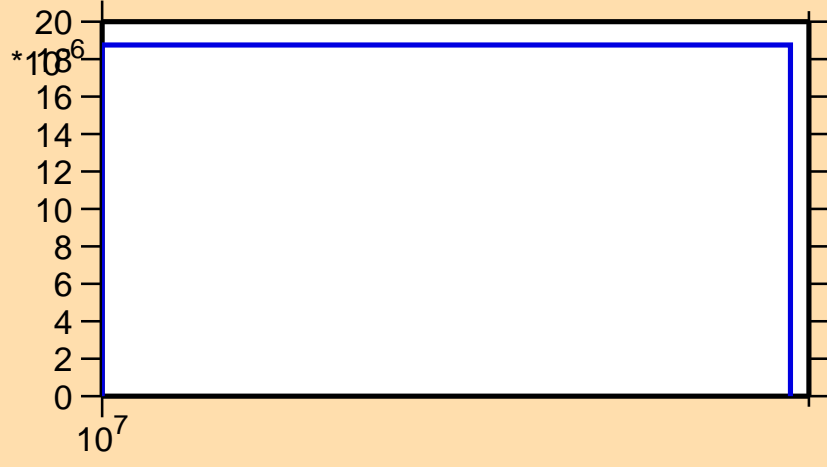
\sigma vs. E for ^{120}\text{Ag}(n,d)
