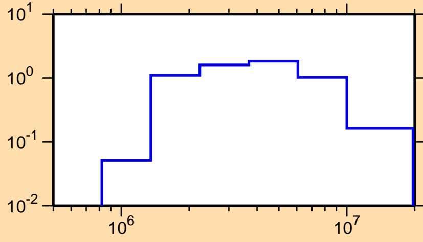
\sigma vs. E for ^{120}\text{Ag}(n,n\text{cont.})
