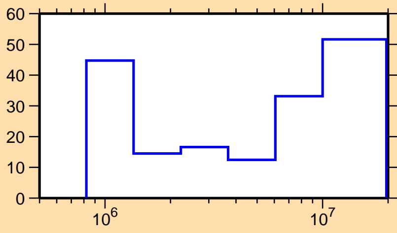
\Delta\sigma/\sigma vs. E for ^{120}\text{Ag}(n,n\text{cont.})
