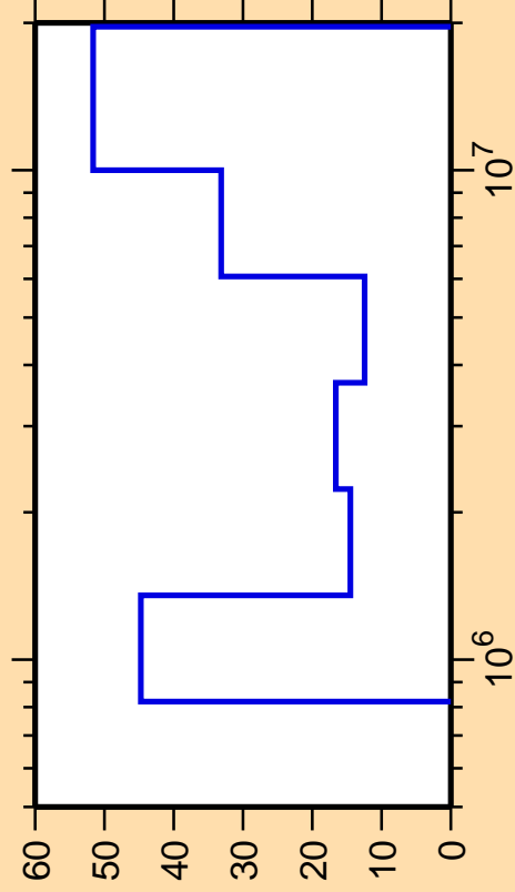
\Delta\sigma/\sigma vs. E for ^{120}\text{Ag}(n,n\text{cont.})
