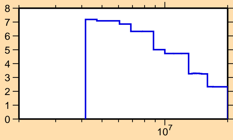
\Delta\sigma/\sigma vs. E for ^{24}\text{Al}(n, tot.)
