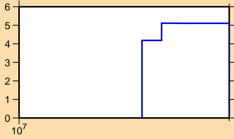
\Delta\sigma/\sigma vs. E for ^{24}\text{Al}(n,\text{el.})
