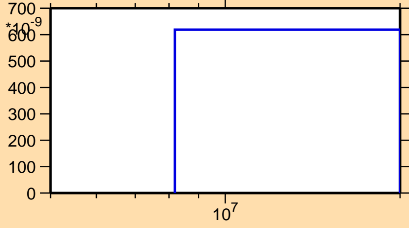
\sigma vs. E for ^{24}\text{Al}(n,2n)
