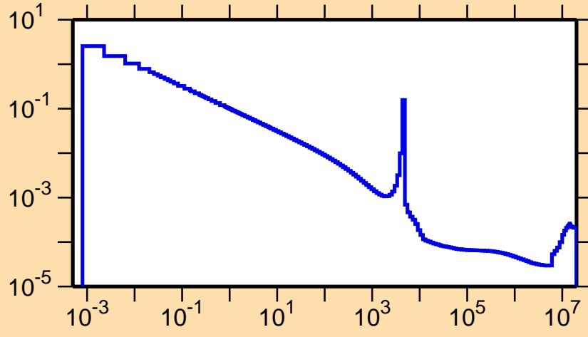
\sigma vs. E for ^{25}\text{Al}(n,\gamma)
