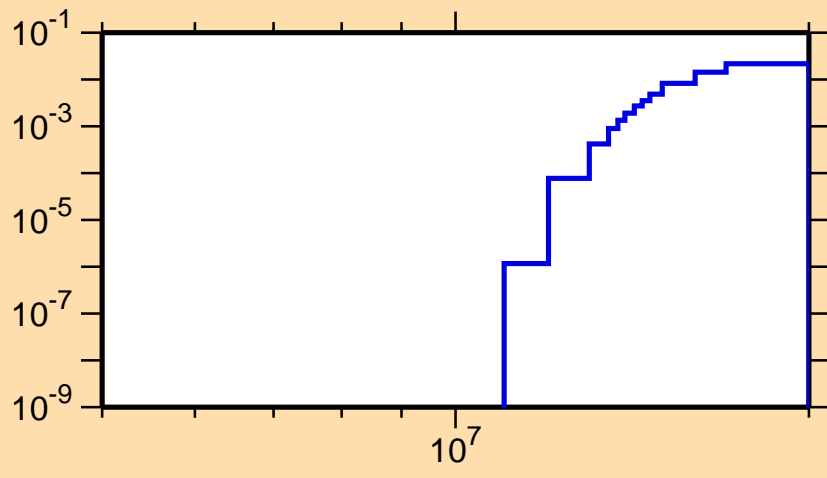
\sigma vs. E for ^{25}\text{Al}(n,n\alpha)
