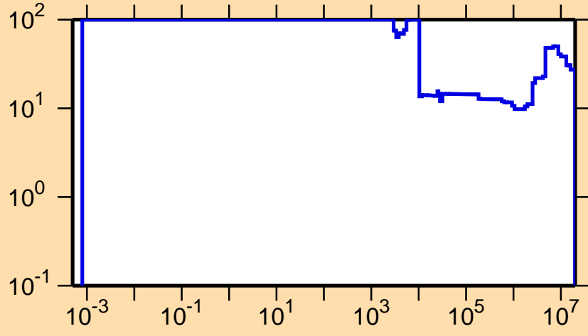
\Delta\sigma/\sigma vs. E for ^{25}\text{Al}(n,p)
