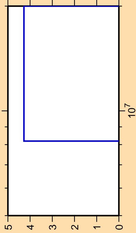
\Delta\sigma/\sigma vs. E for ^{26}\text{Al} (mt 34)
