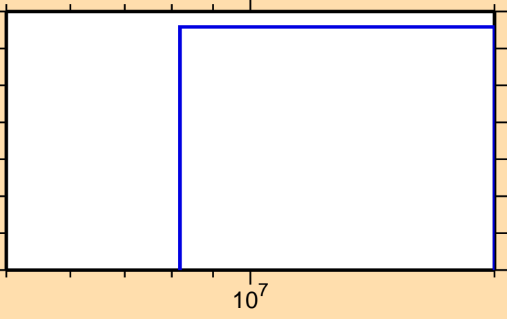
\sigma vs. E for ^{26}\text{Al}(\text{mt117})
