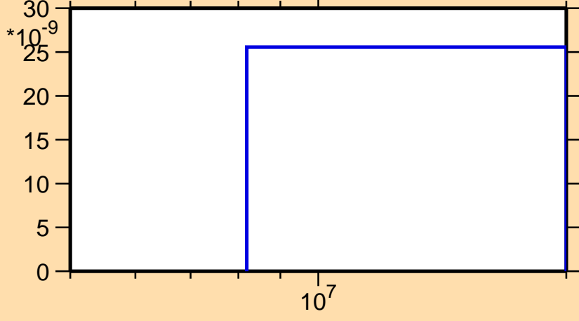
\sigma vs. E for ^{27}\text{Al}(n,\text{nd})
