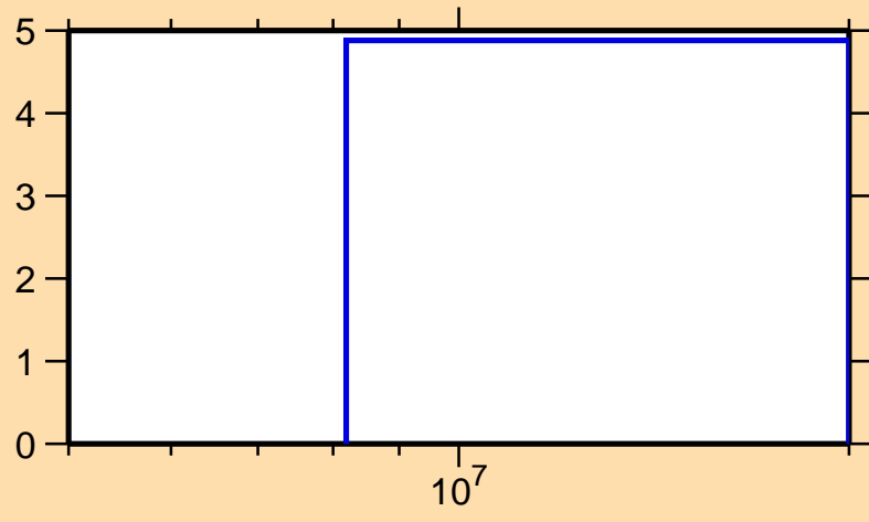
\Delta\sigma/\sigma vs. E for ^{27}\text{Al}(n,\text{inel.})
