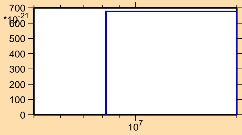
\sigma vs. E for ^{27}\text{Al} (mt 45)
