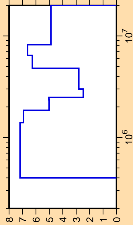
\Delta\sigma/\sigma vs. E for ^{27}\text{Al}(n,\text{inel.})
