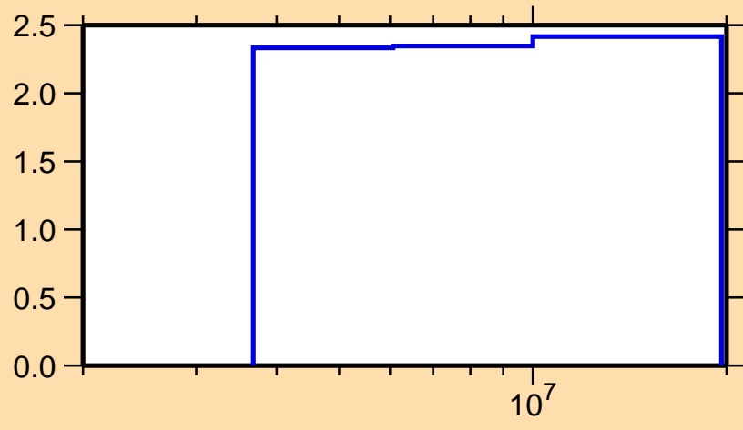
\Delta\sigma/\sigma vs. E for ^{28}\text{Al}(n,n\text{onel.})
