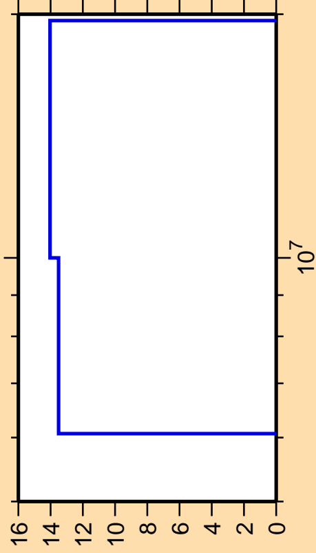
\Delta\sigma/\sigma vs. E for ^{28}\text{Al}(n,t)
