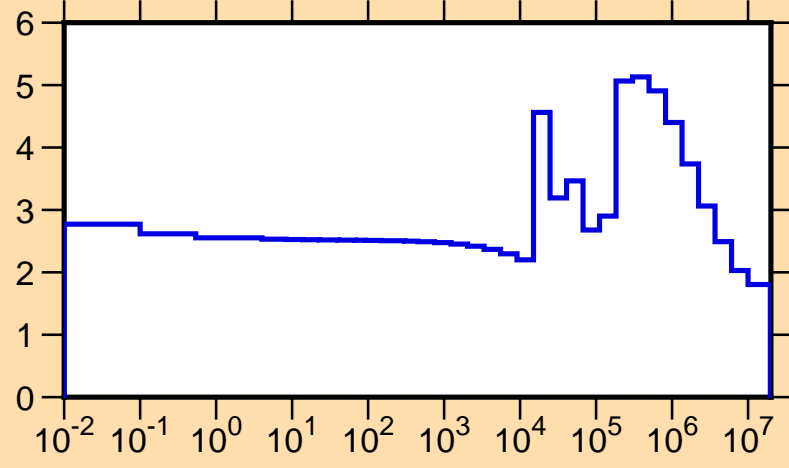
\sigma vs. E for ^{28}\text{Al}(n,\text{tot.})
