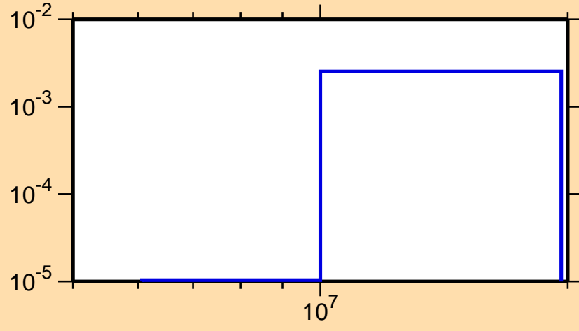
\sigma vs. E for ^{28}\text{Al}(n,t)
