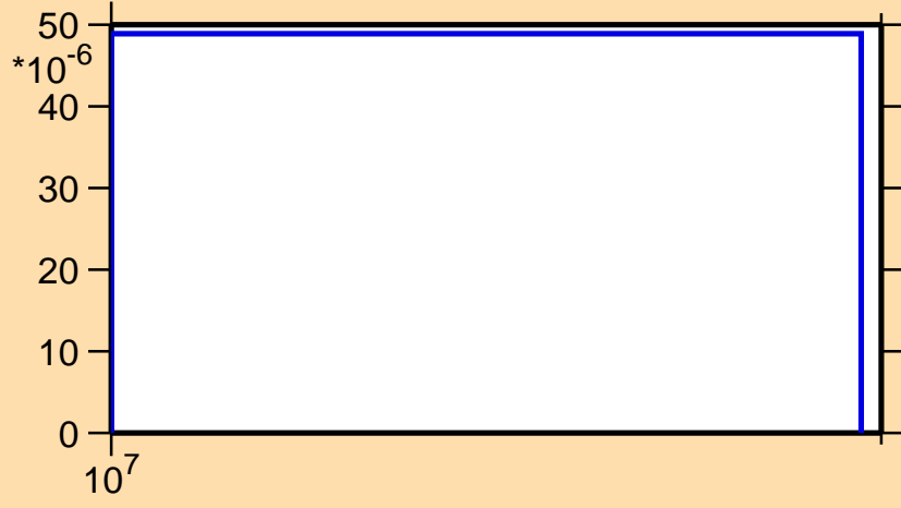
\sigma vs. E for ^{28}\text{Al}(n,\text{nd})
