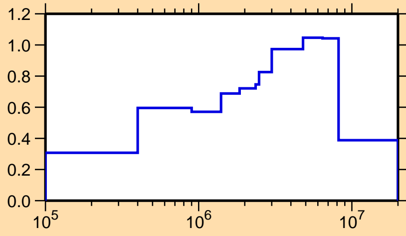
\sigma vs. E for ^{28}\text{Al}(n,\text{inel.})
