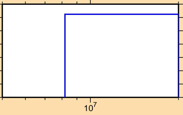
\sigma vs. E for ^{28}\text{Al}(n,2np)
