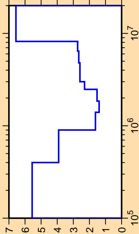
\Delta\sigma/\sigma vs. E for ^{28}\text{Al}(n,\text{inel.})
