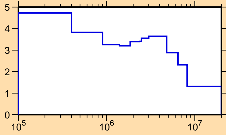
\Delta\sigma/\sigma vs. E for ^{28}\text{Al}(n,\text{tot.})
