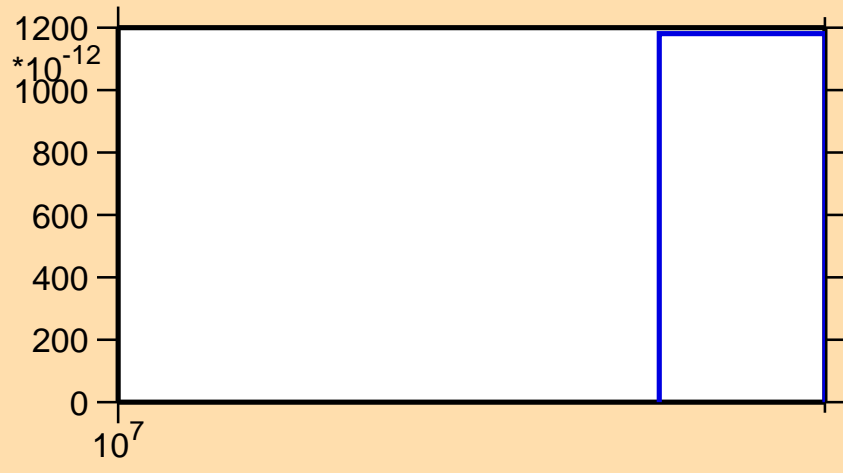
\sigma vs. E for ^{30}\text{Al}(n,2n\alpha)
