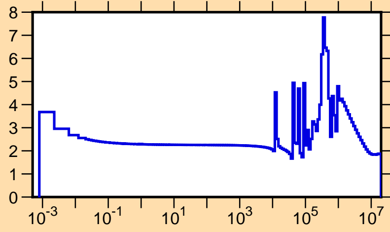
\sigma vs. E for ^{30}\text{Al}(n,\text{tot.})
