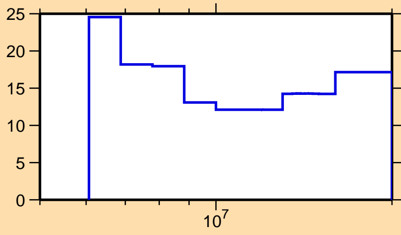
\Delta\sigma/\sigma vs. E for ^{30}\text{Al}(n,2n)
