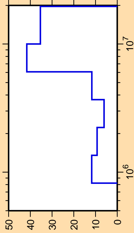
\Delta\sigma/\sigma vs. E for ^{30}\text{Al}(n,n_2)
