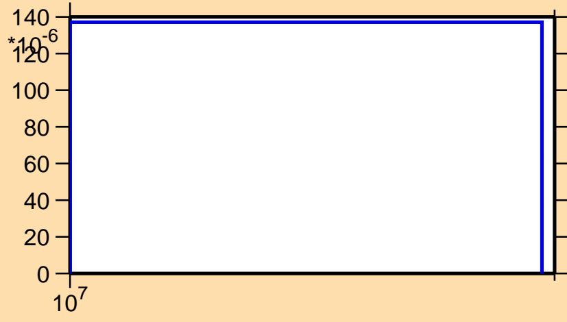
\sigma vs. E for ^{30}\text{Al}(n,n\alpha)
