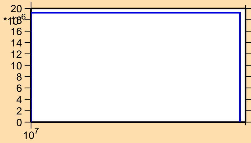
\sigma vs. E for ^{30}\text{Al}(n,nd)
