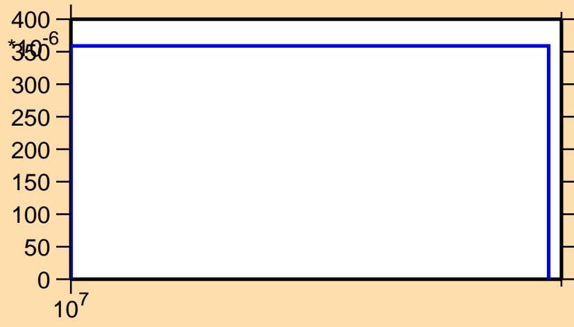
\sigma vs. E for ^{30}\text{Al}(n,np)
