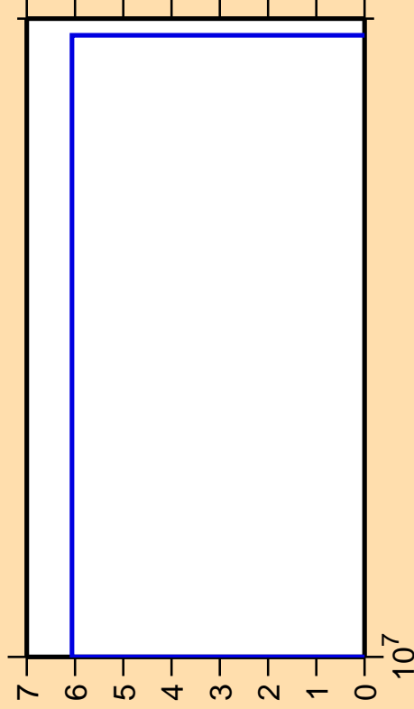
\Delta\sigma/\sigma vs. E for ^{30}\text{Al}(n,2n\alpha)
