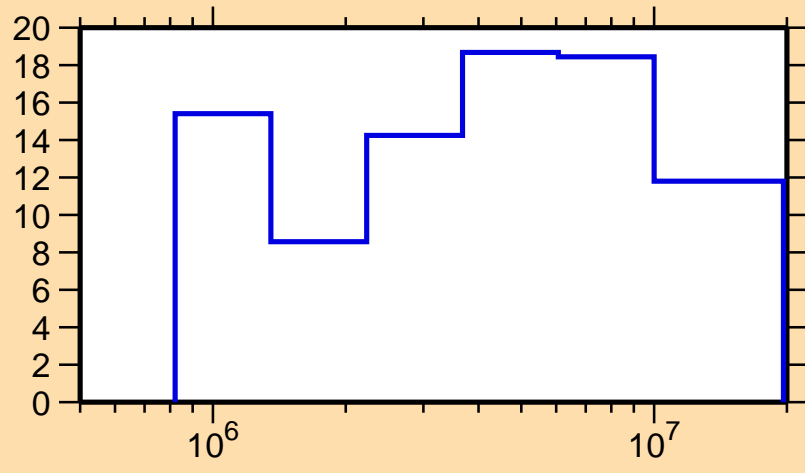
\Delta\sigma/\sigma vs. E for ^{30}\text{Al}(n,\text{el.})
