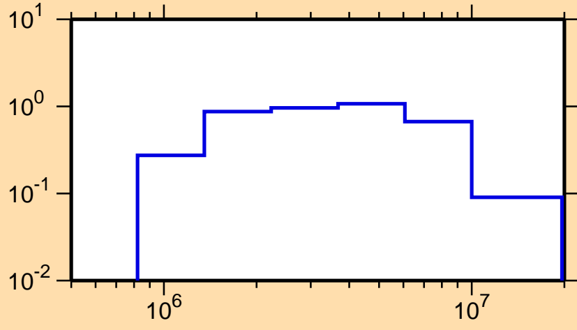
\sigma vs. E for ^{30}\text{Al}(n,\text{inel.})
