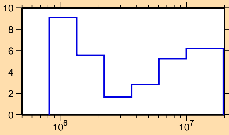
\Delta\sigma/\sigma vs. E for ^{30}\text{Al}(n,\text{nonel.})
