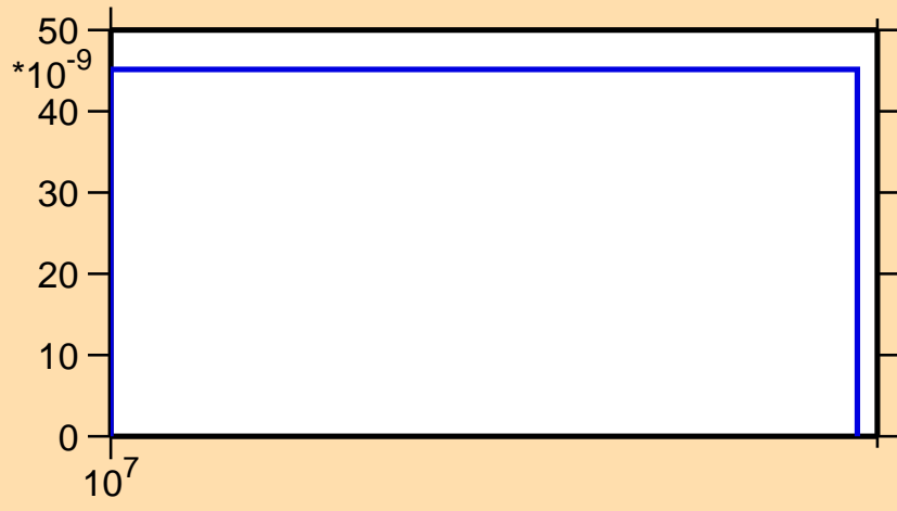
\sigma vs. E for ^{30}\text{Al}(n,nt)
