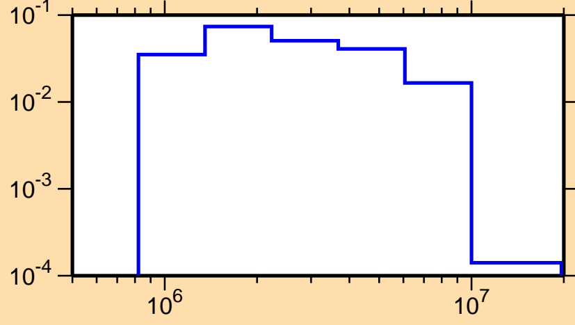
\sigma vs. E for ^{30}\text{Al}(n,n_2)
