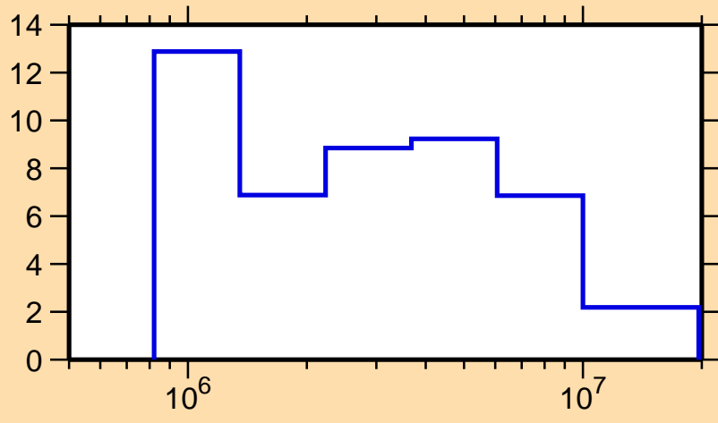
\Delta\sigma/\sigma vs. E for ^{30}\text{Al}(n,\text{tot.})
