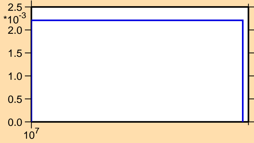
\sigma vs. E for ^{30}\text{Al}(n,d)
