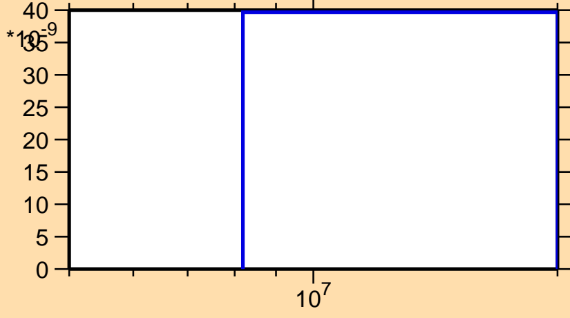
\sigma vs. E for ^{30}\text{Al}(n,2np)
