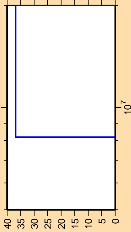
\Delta\sigma/\sigma vs. E for ^{30}\text{Al}(n,nt)
