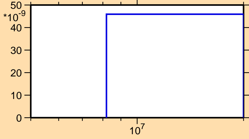
\sigma vs. E for ^{30}\text{Al}(n,nt)
