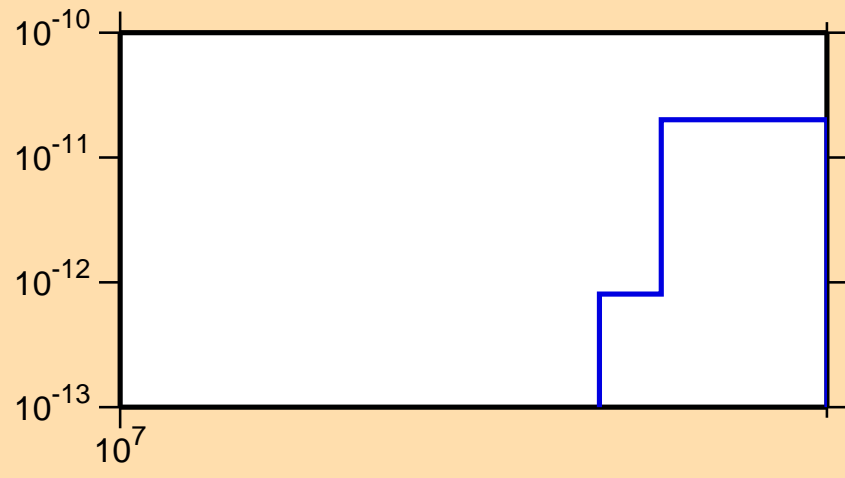
\sigma vs. E for ^{230}\text{Am}(n,nt)
