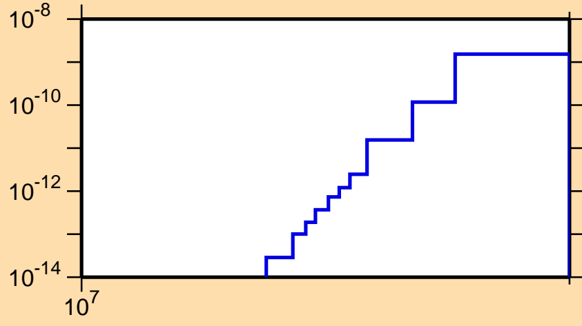
\sigma vs. E for ^{230}\text{Am}(n,2np)
