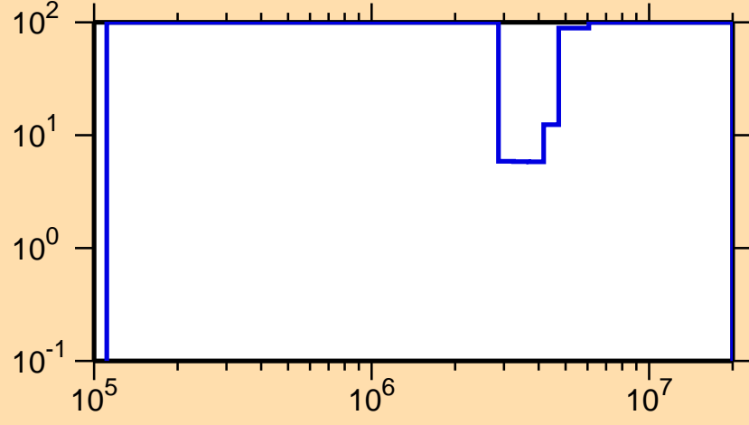
\Delta\sigma/\sigma vs. E for ^{230}\text{Am}(n,n\text{cont.})
