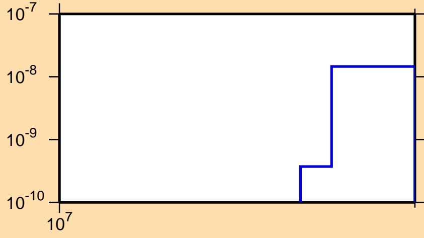
\sigma vs. E for ^{230}\text{Am}(n,3n\alpha)
