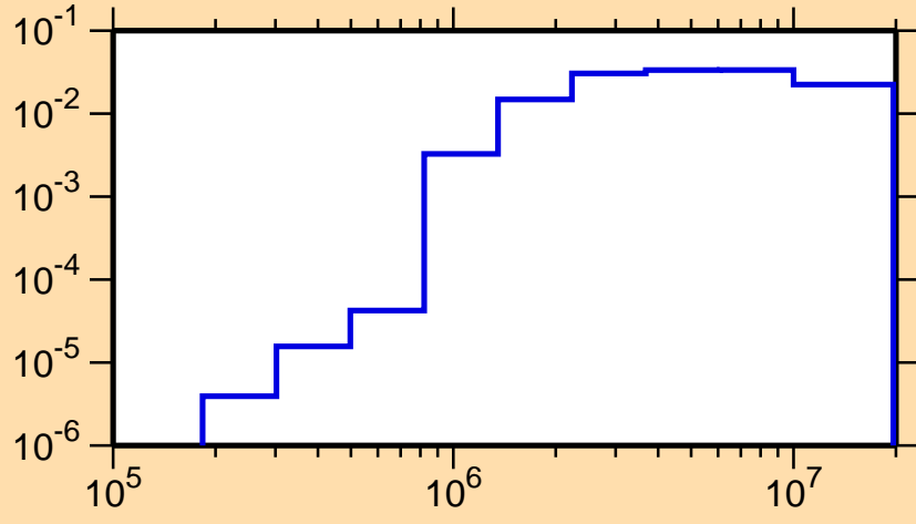
\sigma vs. E for ^{230}\text{Am}(n,n\text{cont.})
