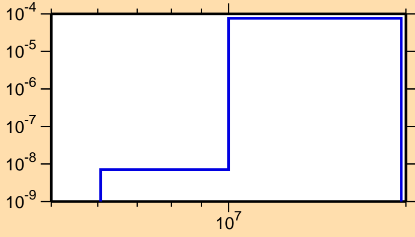
\sigma vs. E for ^{230}\text{Am}(n,t)
