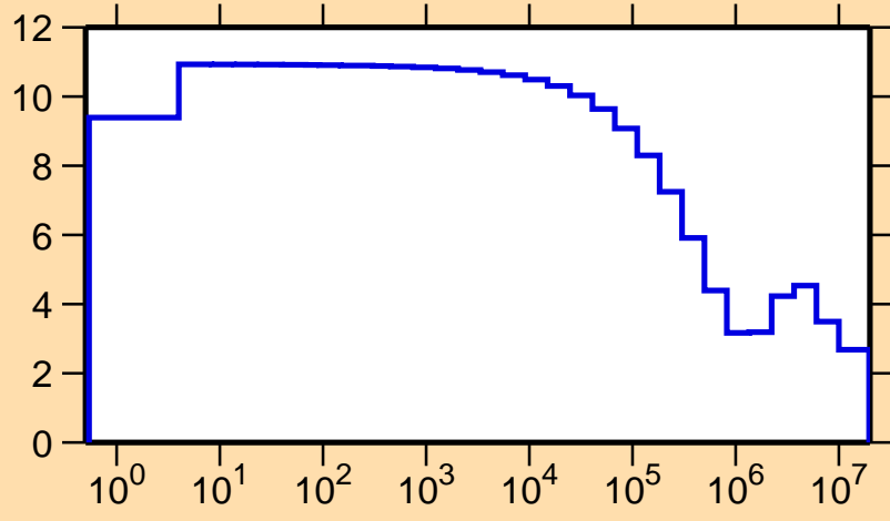
\sigma vs. E for ^{230}\text{Am}(n,\text{el.})
