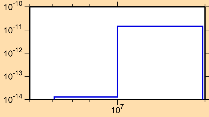
\sigma vs. E for ^{230}\text{Am}(\text{mt117})
