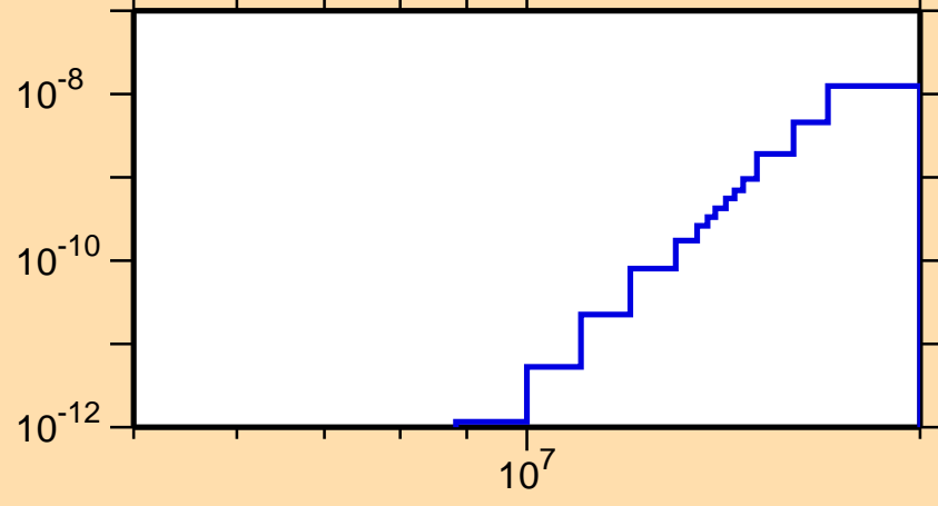
\sigma vs. E for ^{231}\text{Am}(n,p\alpha)
