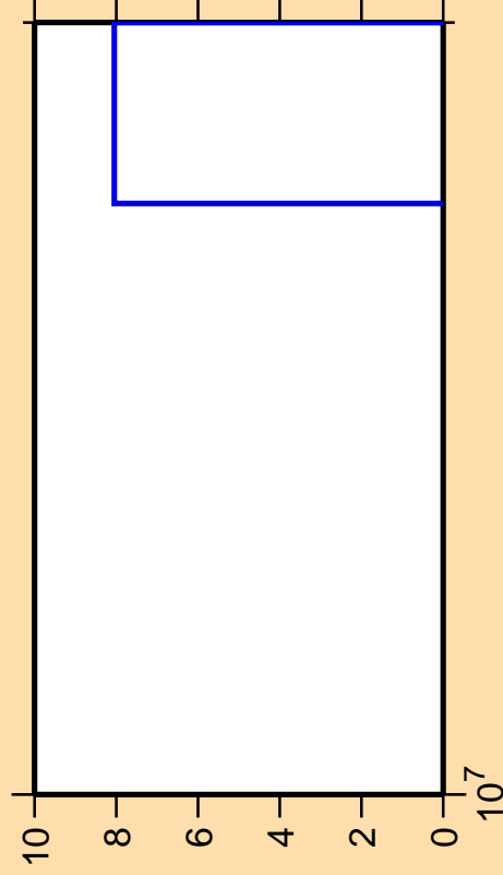
\Delta\sigma/\sigma vs. E for ^{231}\text{Am} (mt 34)
