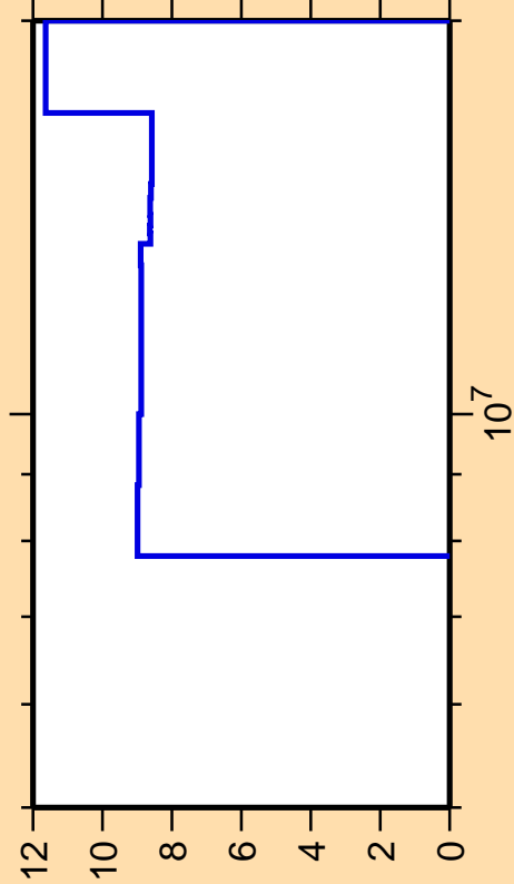
\Delta\sigma/\sigma vs. E for ^{231}\text{Am}(n,f)
