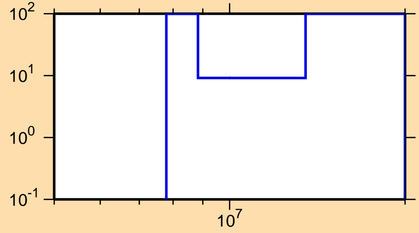
\Delta\sigma/\sigma vs. E for ^{231}\text{Am}(n,2n)
