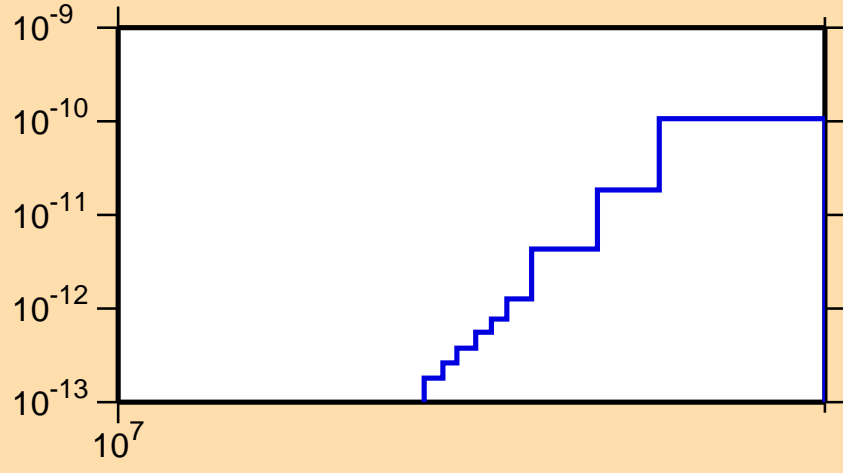
\sigma vs. E for ^{231}\text{Am} (mt 45)
