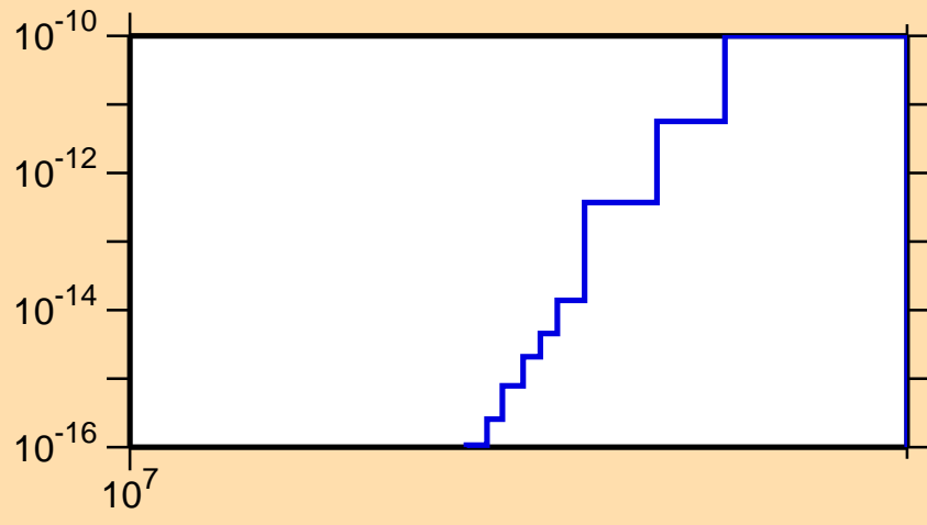
\sigma vs. E for ^{231}\text{Am}(n,2np)
