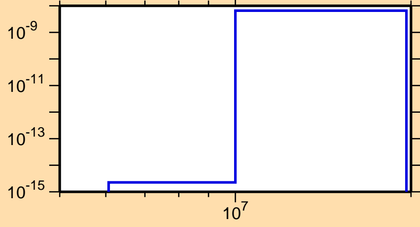
\sigma vs. E for ^{231}\text{Am}(n,2n\alpha)
