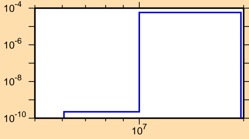
\sigma vs. E for ^{231}\text{Am}(n,t)
