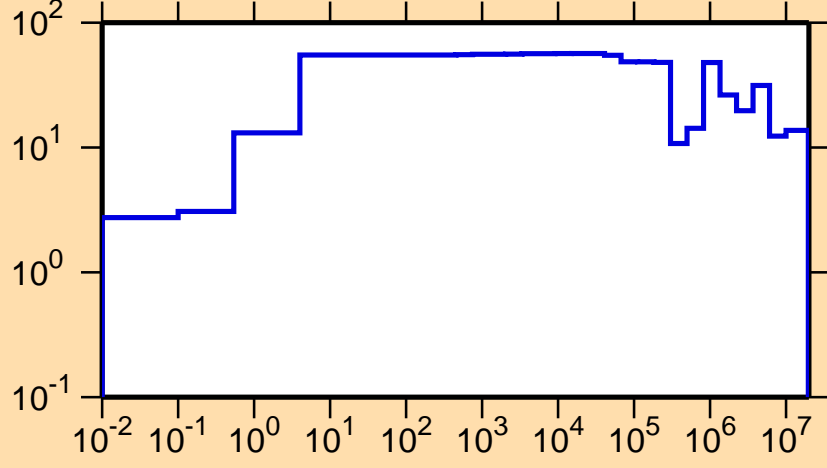
\Delta\sigma/\sigma vs. E for ^{231}\text{Am}(n,\text{el.})
