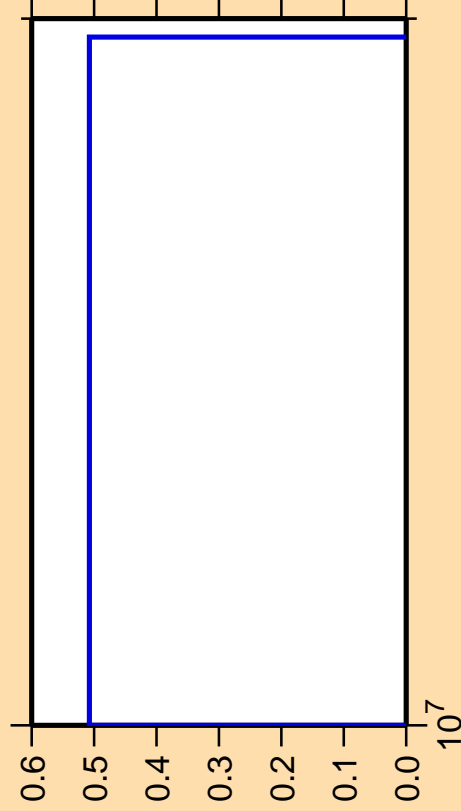
\Delta\sigma/\sigma vs. E for ^{231}\text{Am} (mt 45)
