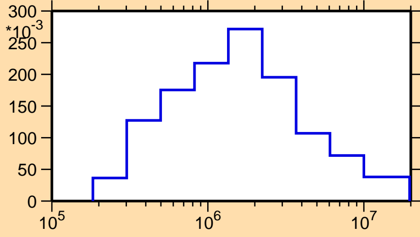
\sigma vs. E for ^{231}\text{Am}(n,n_1)
