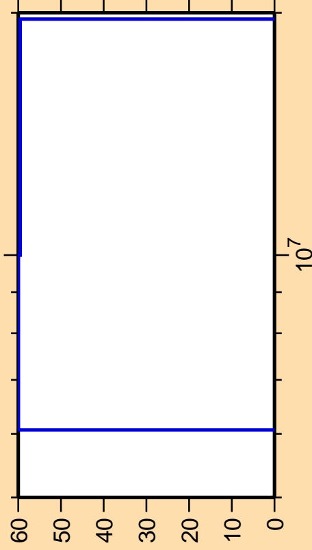
\Delta\sigma/\sigma vs. E for ^{231}\text{Am}(n,\alpha)
