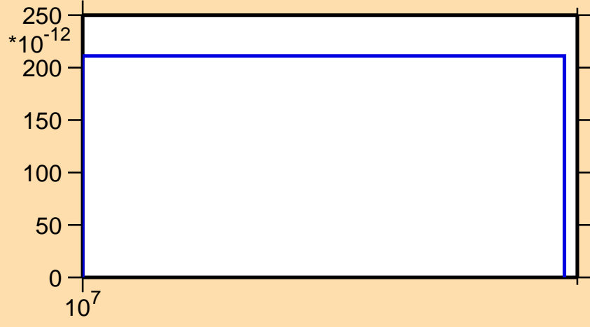
\sigma vs. E for ^{231}\text{Am}(n,3n\alpha)
