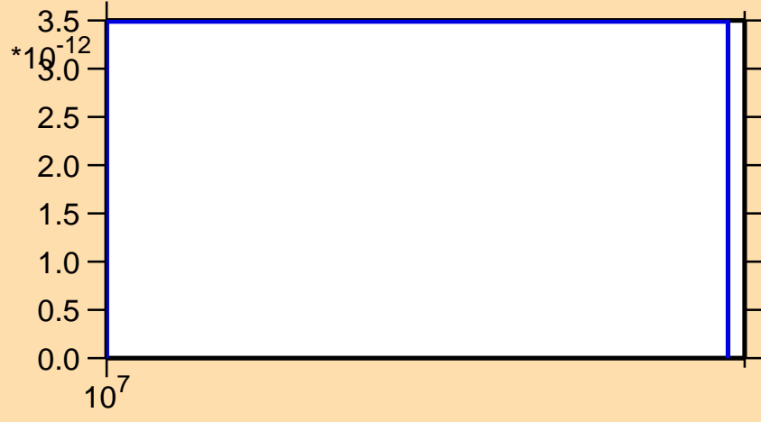
\sigma vs. E for ^{231}\text{Am}(\text{mt117})
