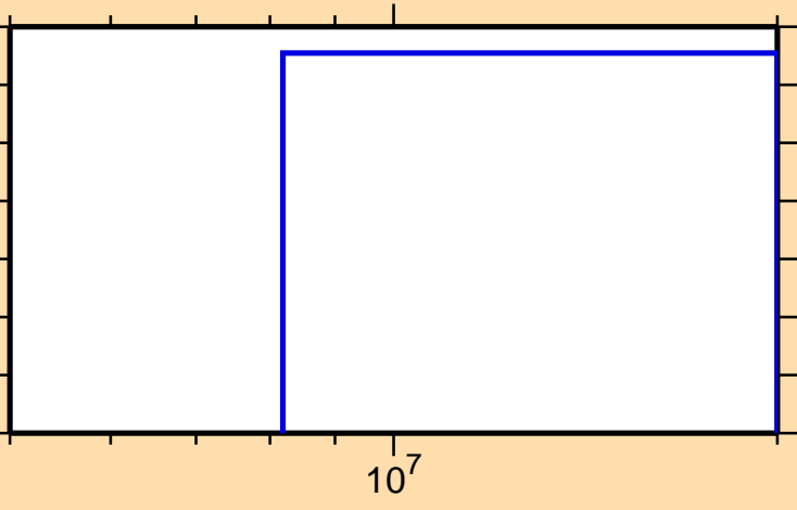
\sigma vs. E for ^{231}\text{Am}(n,\text{He}3)
