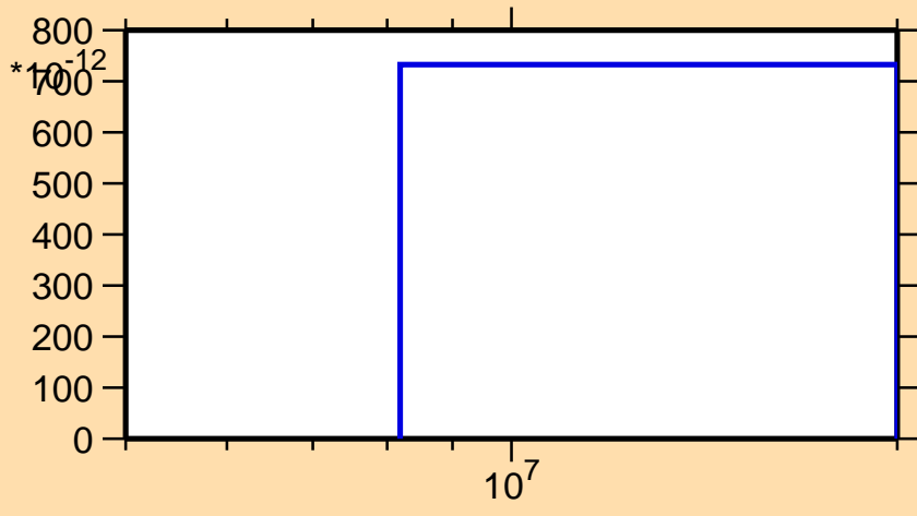
\sigma vs. E for ^{231}\text{Am}(n,p\alpha)
