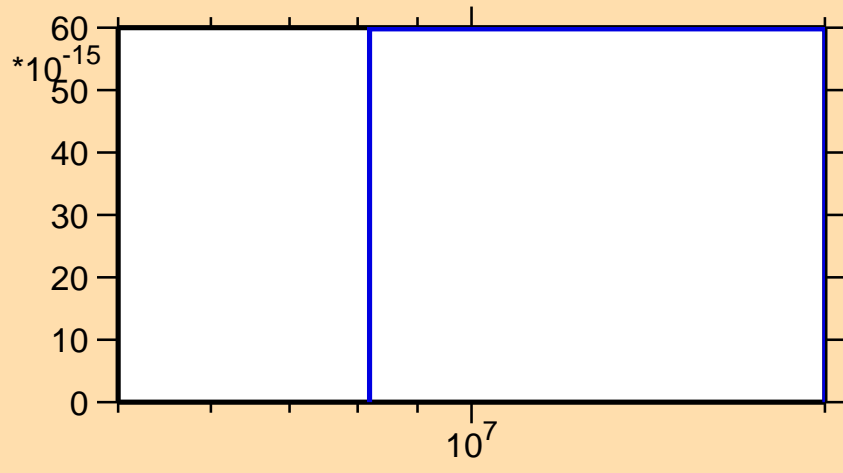
\sigma vs. E for ^{231}\text{Am} (mt 34)
