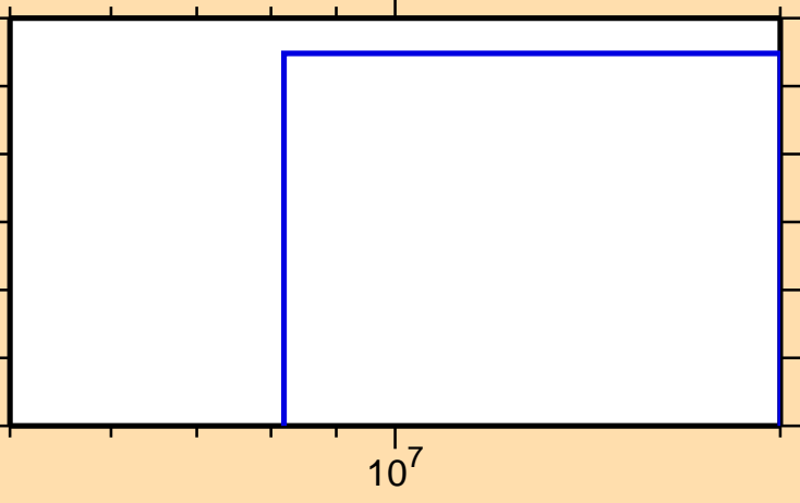
\sigma vs. E for ^{231}\text{Am}(n,2n\alpha)
