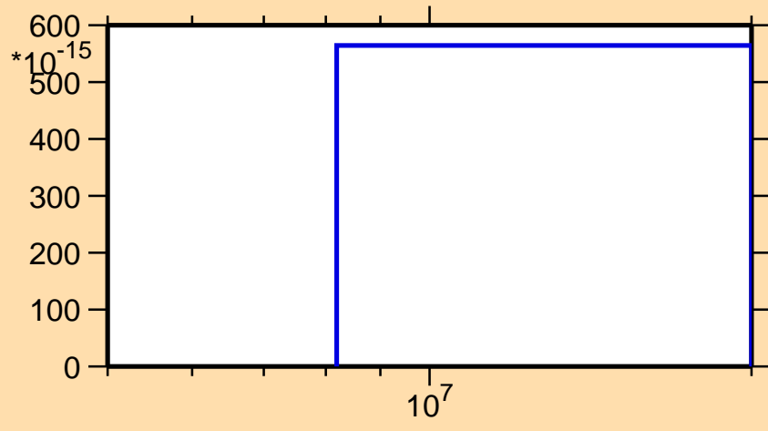
\sigma vs. E for ^{231}\text{Am}(n,nt)
