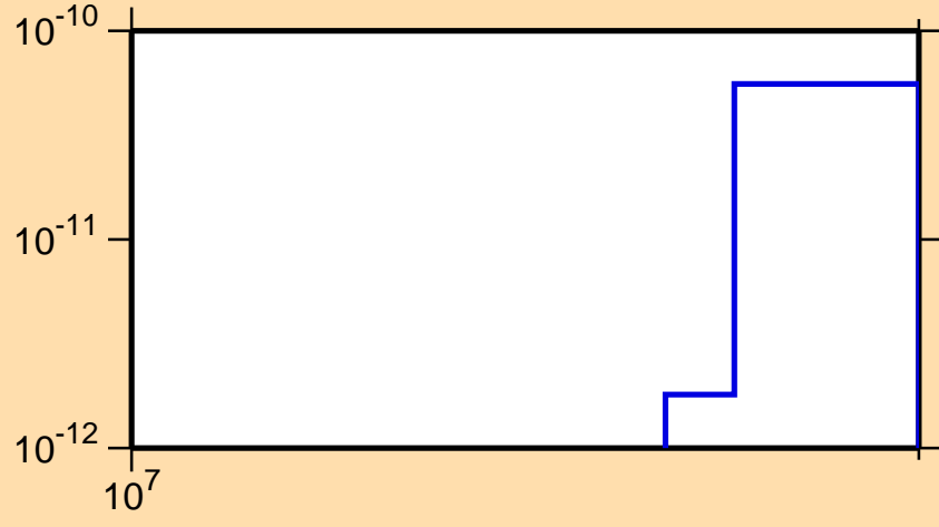
\sigma vs. E for ^{232}\text{Am}(n,nt)
