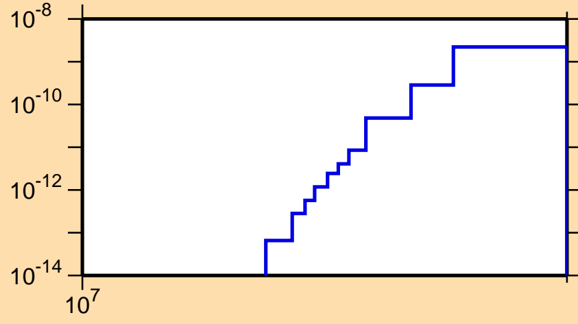
\sigma vs. E for ^{232}\text{Am}(n,2np)
