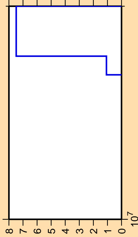
\Delta\sigma/\sigma vs. E for ^{233}\text{Am} (mt 45)
