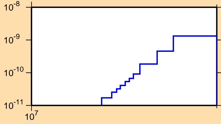
\sigma vs. E for ^{233}\text{Am}(n,p\alpha)
