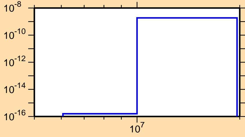
\sigma vs. E for ^{233}\text{Am}(n,\text{He3})
