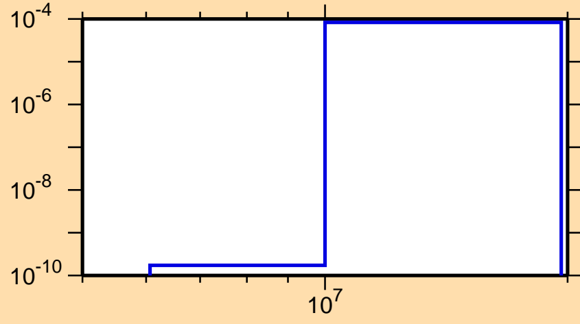
\sigma vs. E for ^{233}\text{Am}(n,t)
