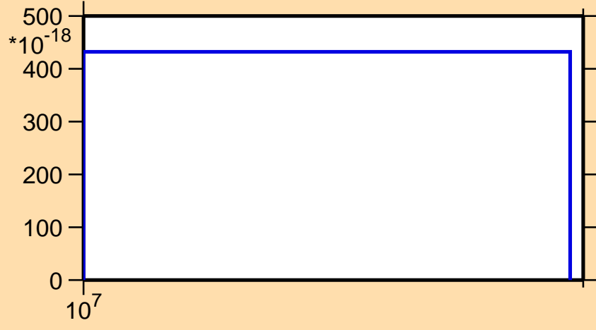
\sigma vs. E for ^{233}\text{Am}(n,3n\alpha)
