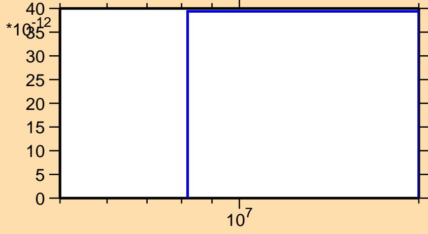
\sigma vs. E for ^{233}\text{Am}(n,2np)
