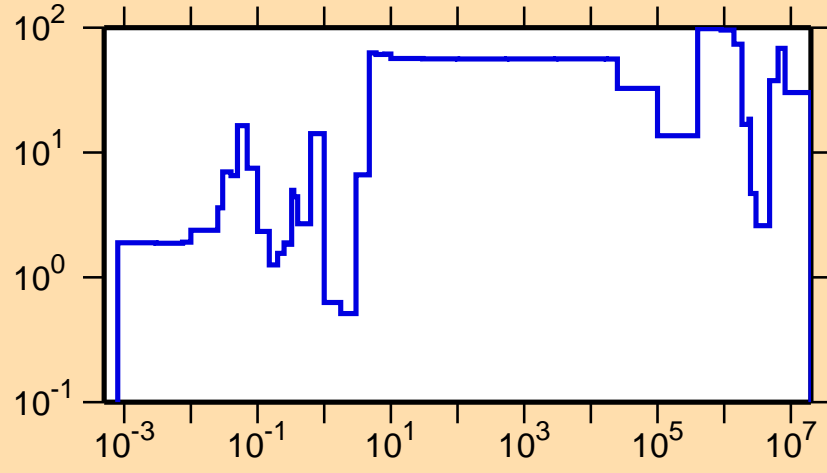
\Delta\sigma/\sigma vs. E for ^{233}\text{Am}(n,el.)
