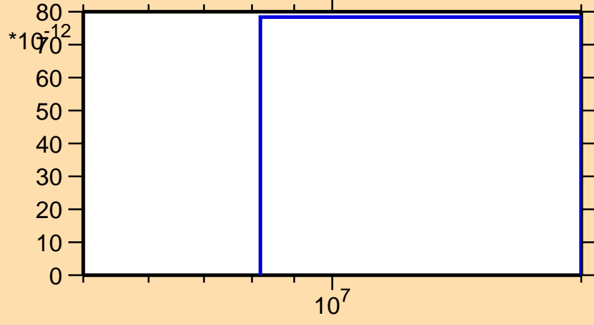
\sigma vs. E for ^{233}\text{Am}(n,\text{nd})
