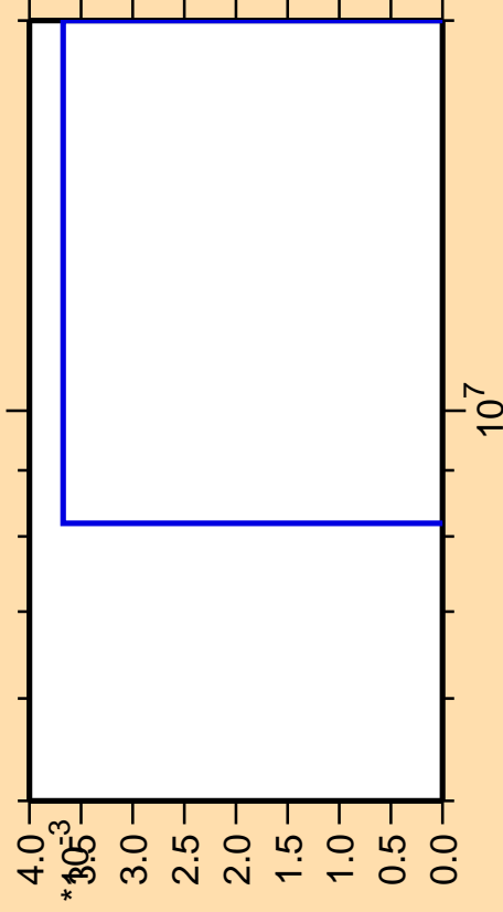
\Delta\sigma/\sigma vs. E for ^{233}\text{Am}(n,3n\alpha)
