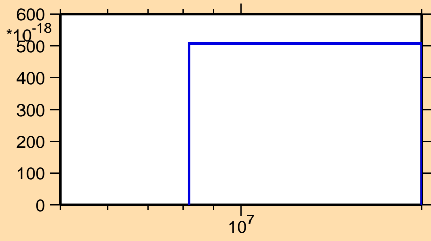
\sigma vs. E for ^{233}\text{Am}(n,3n\alpha)
