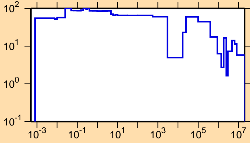
\Delta\sigma/\sigma vs. E for ^{233}\text{Am}(n,p)
