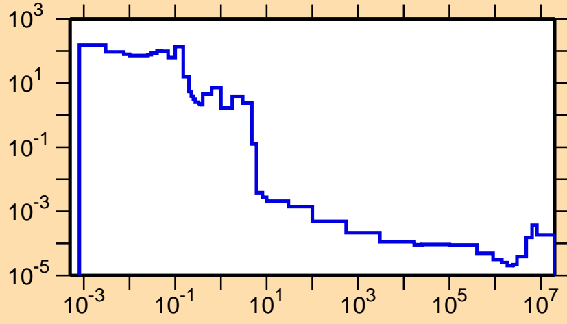
\sigma vs. E for ^{233}\text{Am}(n,\gamma)
