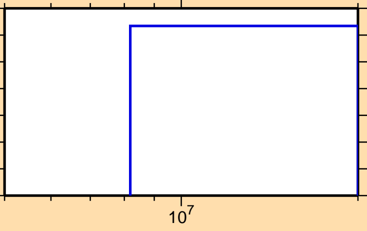
\sigma vs. E for ^{233}\text{Am}(n,2n\alpha)
