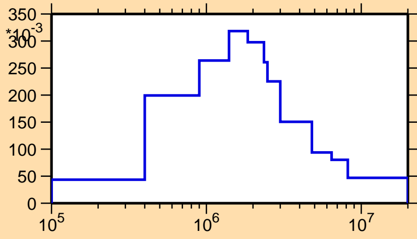
\sigma vs. E for ^{233}\text{Am}(n,\text{inel.})
