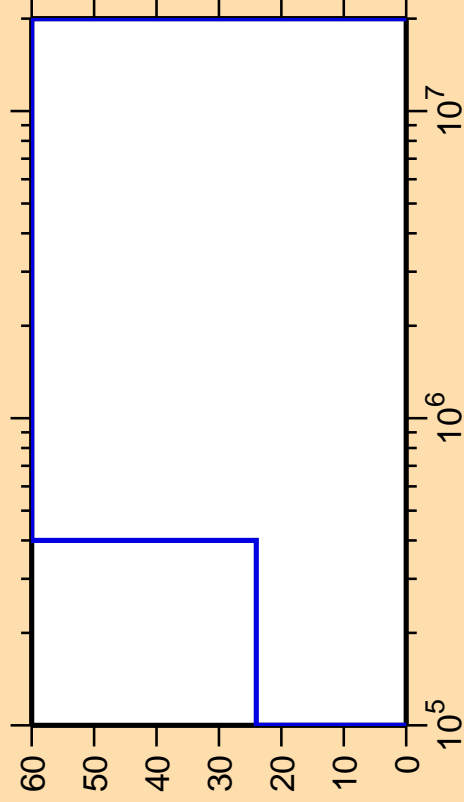
\Delta\sigma/\sigma vs. E for ^{233}\text{Am}(n,\text{inel.})
