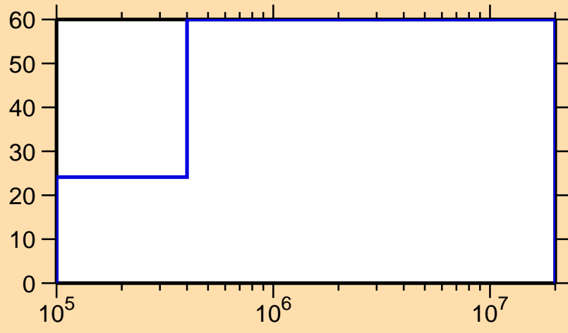
\Delta\sigma/\sigma vs. E for ^{233}\text{Am}(n,n_1)
