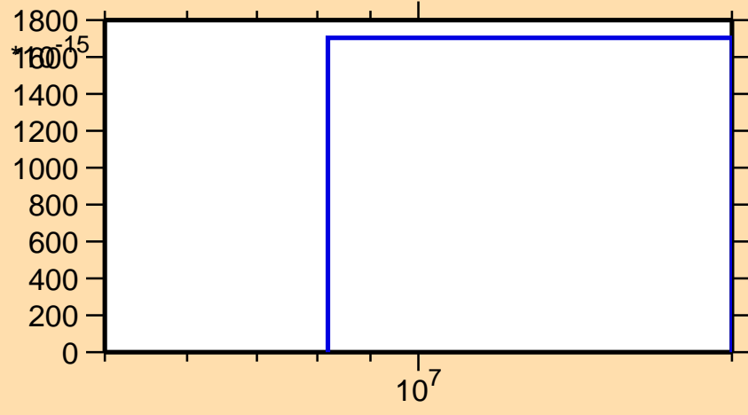
\sigma vs. E for ^{233}\text{Am}(n,nt)
