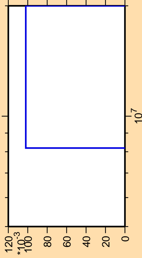
\Delta\sigma/\sigma vs. E for ^{233}\text{Am} (mt 45)
