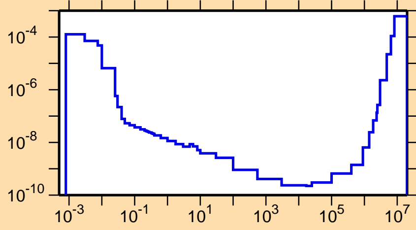
\sigma vs. E for ^{233}\text{Am}(n,p)
