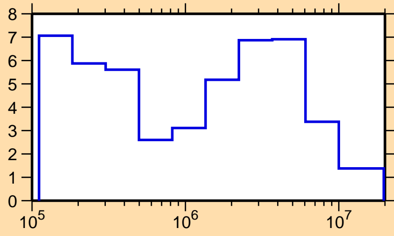
\Delta\sigma/\sigma vs. E for ^{234}\text{Am}(n,\text{tot.})
