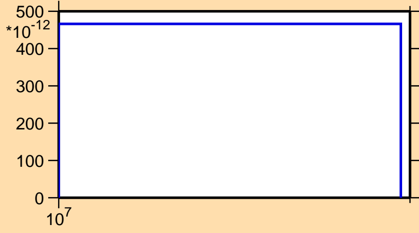
\sigma vs. E for ^{234}\text{Am}(n,2np)
