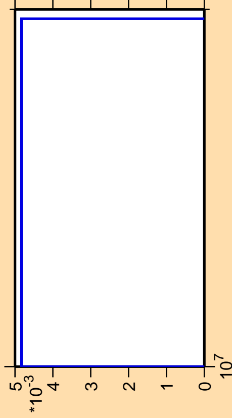
\Delta\sigma/\sigma vs. E for ^{234}\text{Am}(n,3n\alpha)
