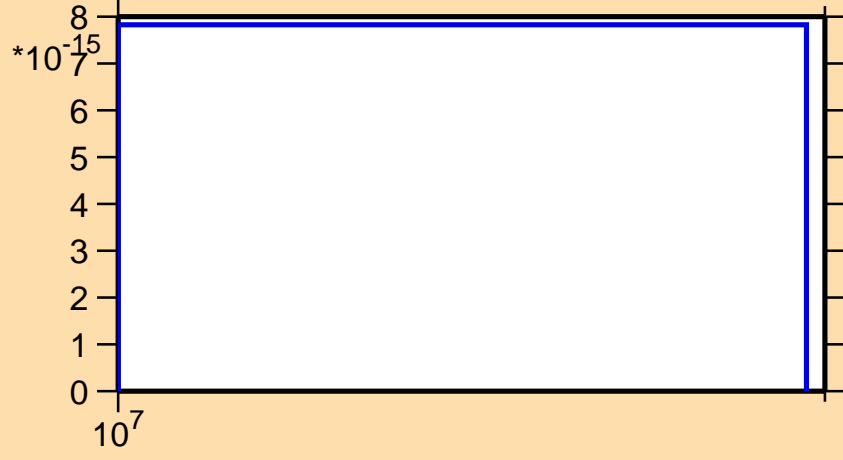
\sigma vs. E for ^{234}\text{Am}(n,3n\alpha)
