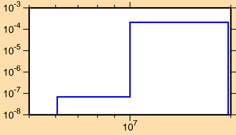
\sigma vs. E for ^{234}\text{Am}(n,d)
