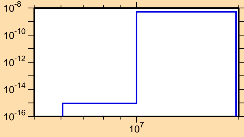
\sigma vs. E for ^{234}\text{Am}(n,\text{He3})
