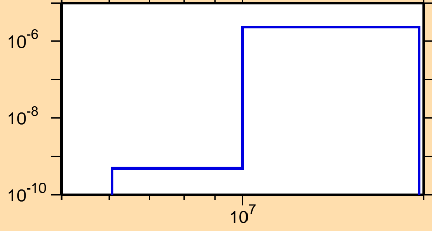
\sigma vs. E for ^{234}\text{Am}(n,t)
