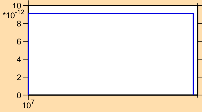
\sigma vs. E for ^{234}\text{Am}(n,p\alpha)
