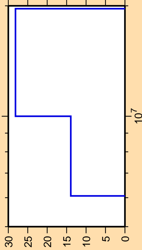
\Delta\sigma/\sigma vs. E for ^{234}\text{Am}(n,d)
