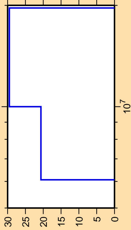
\Delta\sigma/\sigma vs. E for ^{234}\text{Am}(n,np)
