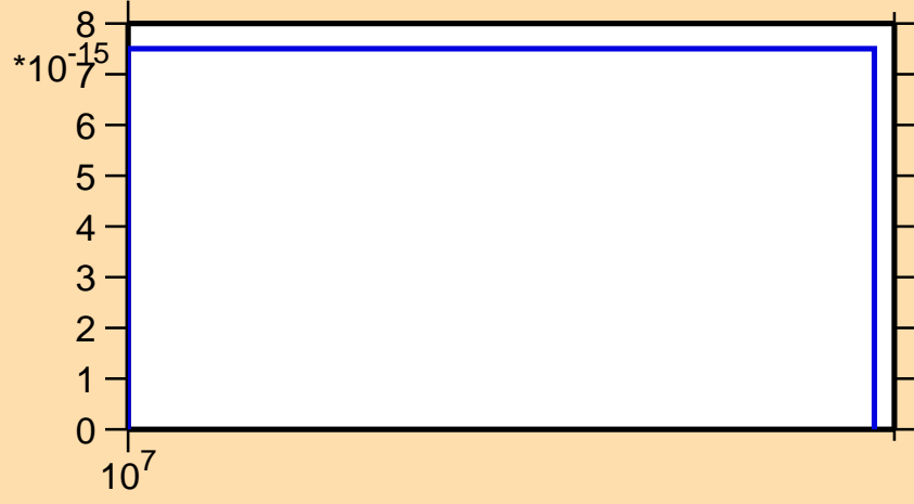
\sigma vs. E for ^{234}\text{Am} (mt 45)
