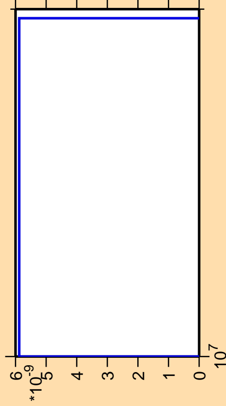
\Delta\sigma/\sigma vs. E for ^{234}\text{Am} (mt 45)
