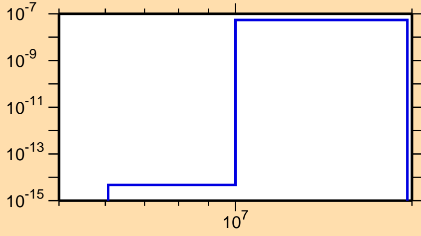
\sigma vs. E for ^{234}\text{Am}(n,2n\alpha)
