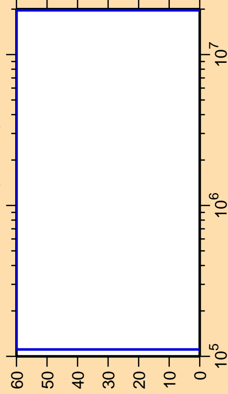
\Delta\sigma/\sigma vs. E for ^{234}\text{Am}(n,\text{inel.})
