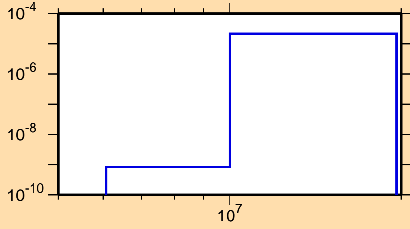
\sigma vs. E for ^{234}\text{Am}(n,np)
