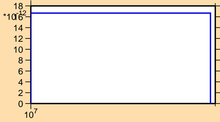
\sigma vs. E for ^{234}\text{Am}(n,nt)
