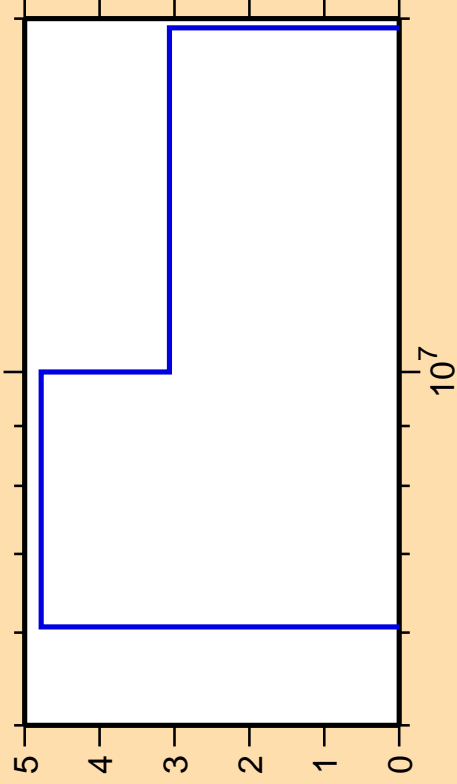
\Delta\sigma/\sigma vs. E for ^{234}\text{Am}(n,f)
