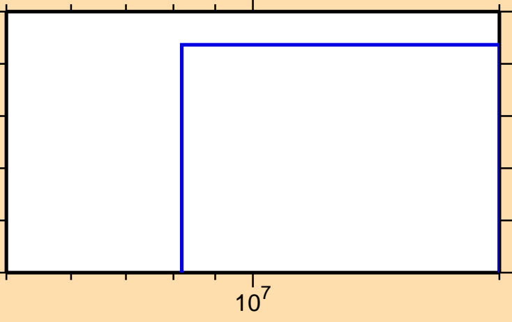
\sigma vs. E for ^{234}\text{Am}(n,3n\alpha)
