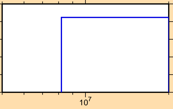
\sigma vs. E for ^{234}\text{Am}(n,\text{He3})
