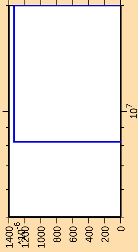
\Delta\sigma/\sigma vs. E for ^{235}\text{Am}(n,3n\alpha)
