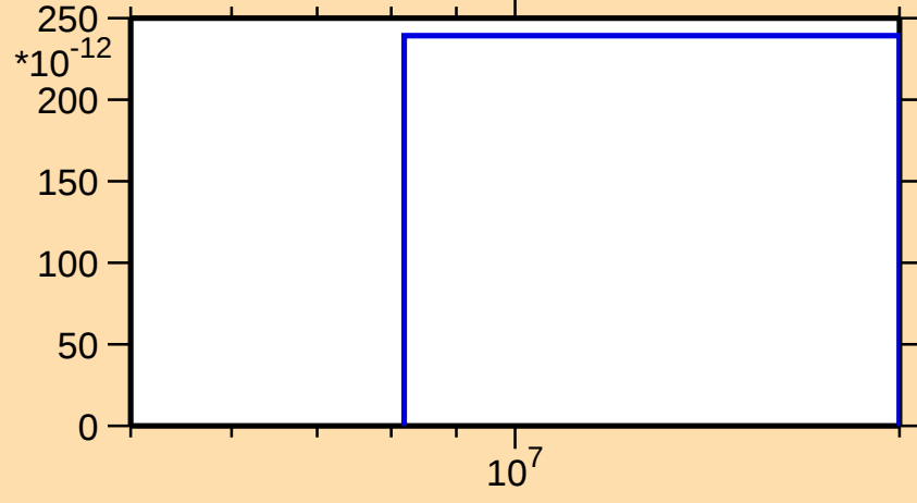
\sigma vs. E for ^{235}\text{Am}(n,\text{He}3)
