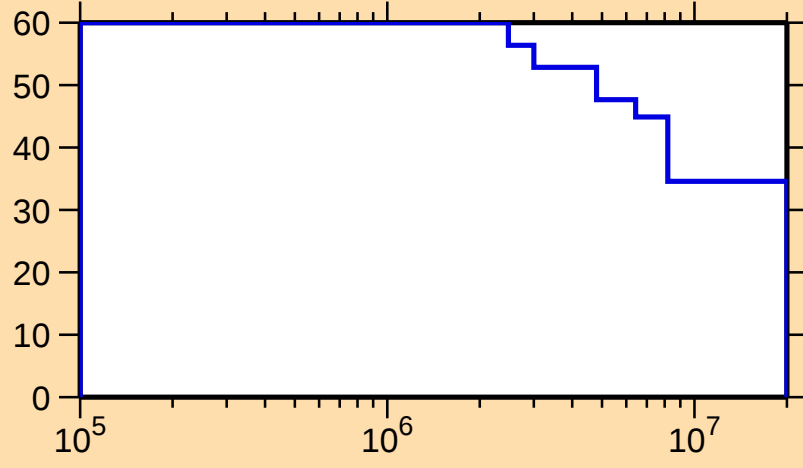
\Delta\sigma/\sigma vs. E for ^{235}\text{Am}(n,n_1)
