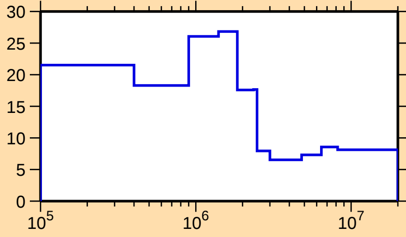
\Delta\sigma/\sigma vs. E for ^{235}\text{Am}(n,f)
