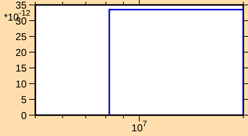
\sigma vs. E for ^{235}\text{Am}(n,nt)
