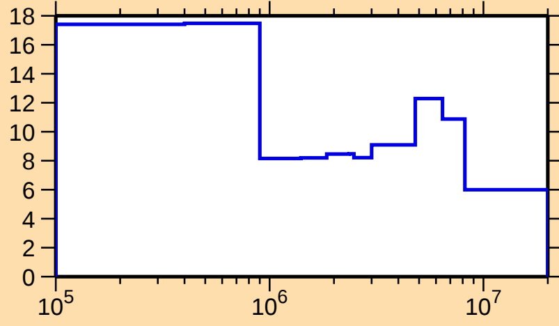
\Delta\sigma/\sigma vs. E for ^{235}\text{Am}(n,\text{tot.})
