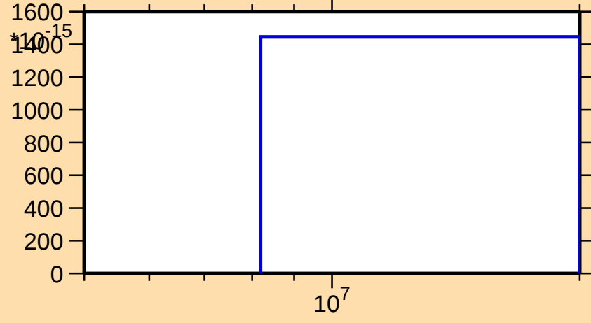
\sigma vs. E for ^{235}\text{Am}(n,p\alpha)
