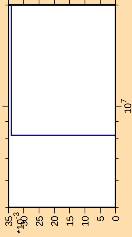
\Delta\sigma/\sigma vs. E for ^{235}\text{Am}(\text{mt } 45)
