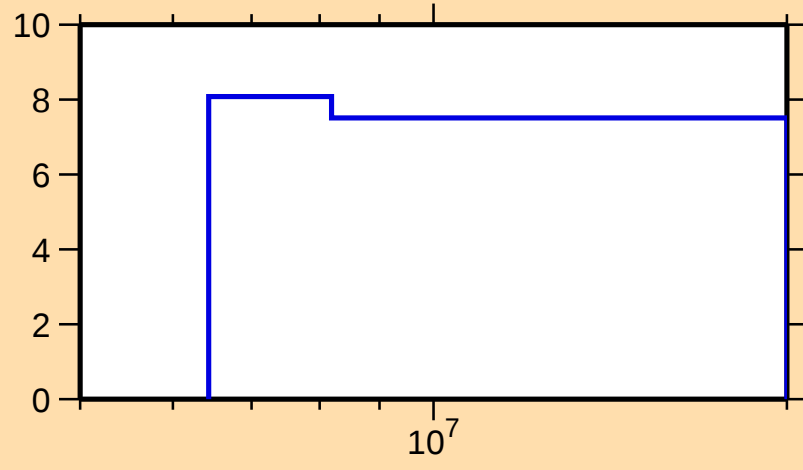
\Delta\sigma/\sigma vs. E for ^{235}\text{Am}(n,\text{nonel.})
