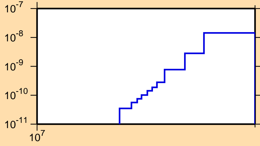
\sigma vs. E for ^{236}\text{Am}(n,2n\alpha)
