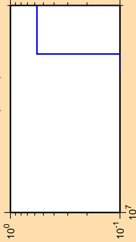
\Delta\sigma/\sigma vs. E for ^{236}\text{Am} (mt 34)
