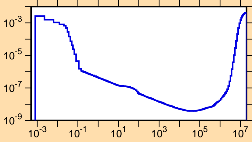
\sigma vs. E for ^{236}\text{Am}(n,p)
