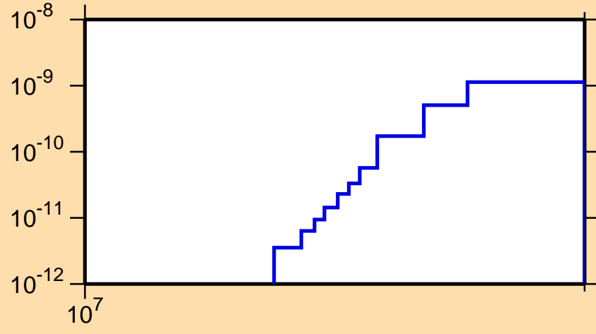
\sigma vs. E for ^{236}\text{Am}(n,t)
