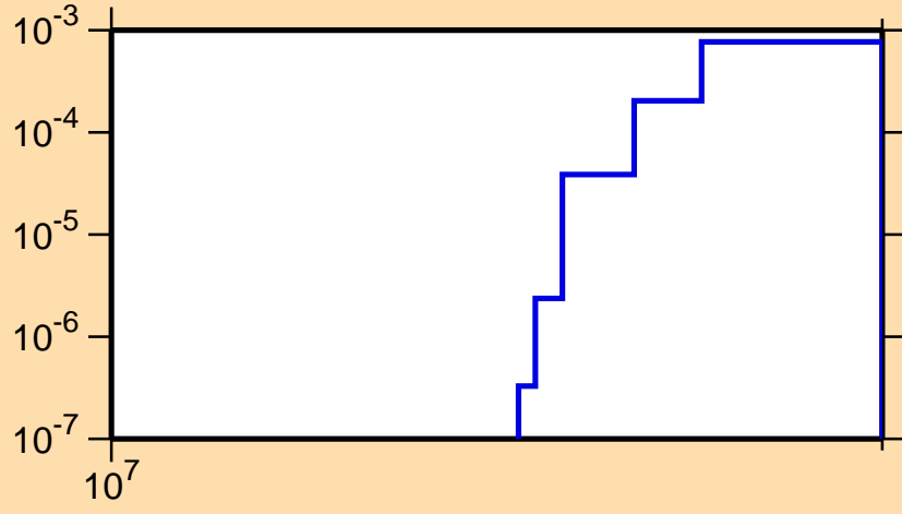
\sigma vs. E for ^{236}\text{Am}(n,3n)
