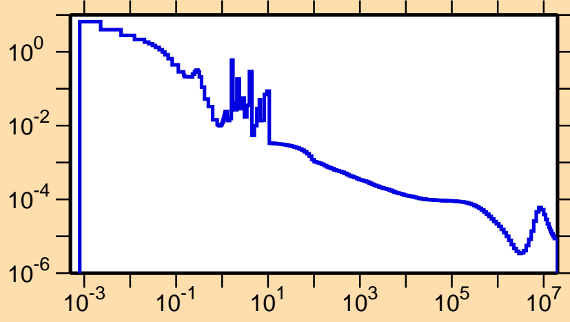
\sigma vs. E for ^{236}\text{Am}(n,\gamma)
