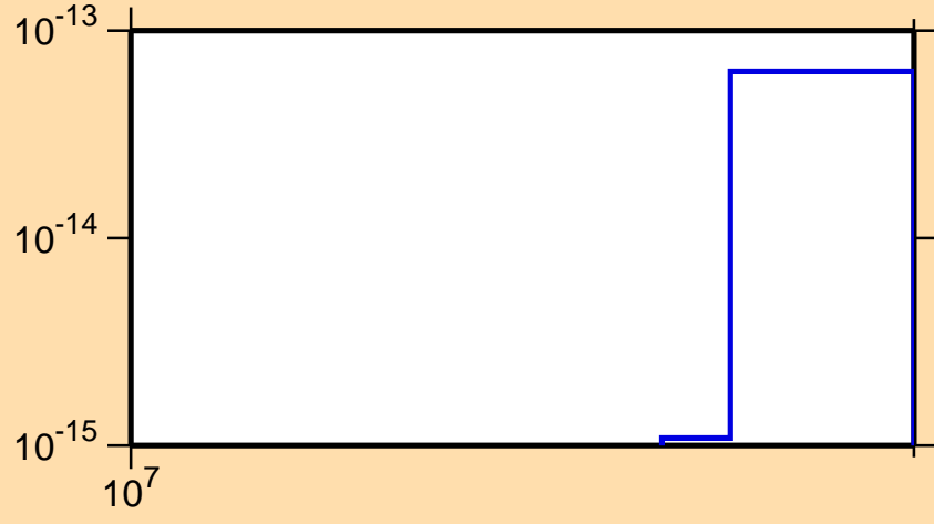
\sigma vs. E for ^{236}\text{Am} (mt 34)
