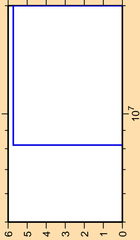
\Delta\sigma/\sigma vs. E for ^{236}\text{Am}(n,p\alpha)
