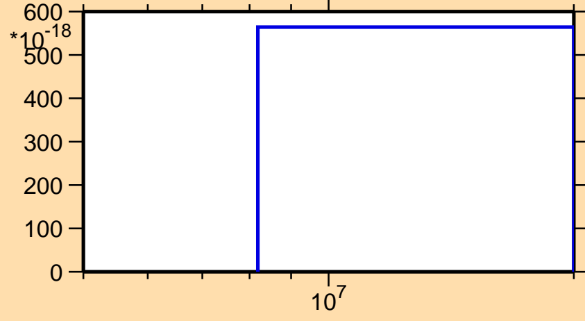
\sigma vs. E for ^{236}\text{Am} (mt 34)
