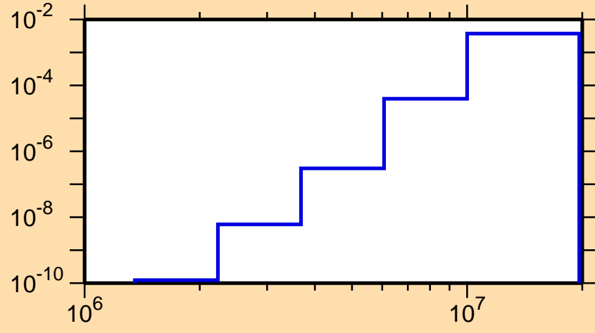
\sigma vs. E for ^{239}\text{Am}(n,p)
