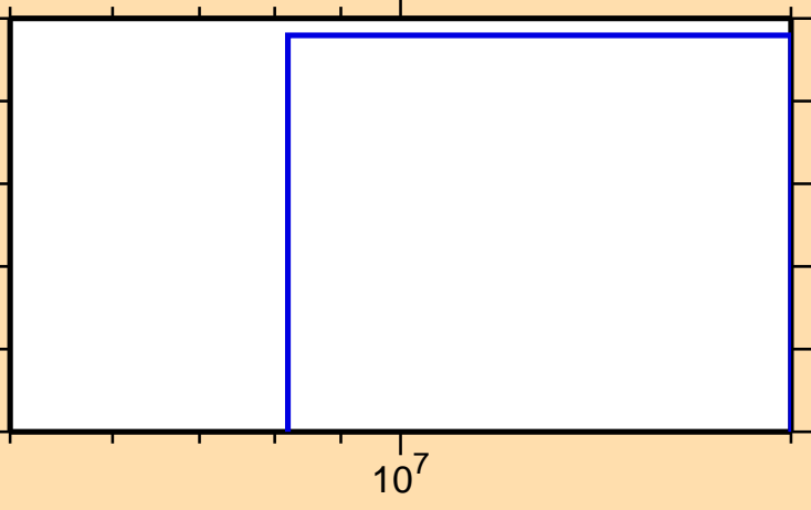
\sigma vs. E for ^{239}\text{Am}(n,3n\alpha)
