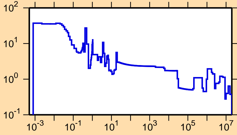
\Delta\sigma/\sigma vs. E for ^{240}\text{Am}(n,el.)
