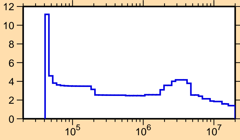
\Delta\sigma/\sigma vs. E for ^{240}\text{Am}(n,n_1)
