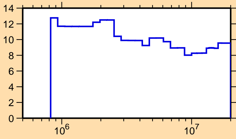
\Delta\sigma/\sigma vs. E for ^{240}\text{Am}(n,n\text{cont.})
