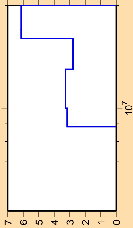
\Delta\sigma/\sigma vs. E for ^{240}\text{Am}(n,t)
