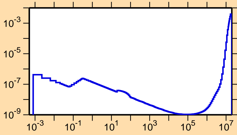
\sigma vs. E for ^{240}\text{Am}(n,\alpha)
