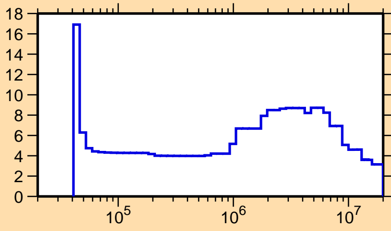
\Delta\sigma/\sigma vs. E for ^{240}\text{Am}(n,\text{inel.})
