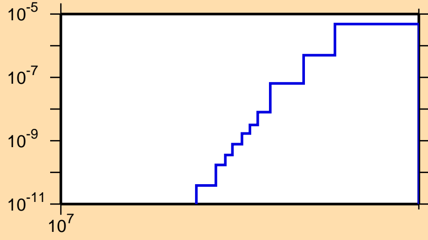
\sigma vs. E for ^{240}\text{Am}(n,\text{nd})
