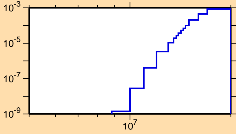
\sigma vs. E for ^{240}\text{Am}(n,t)
