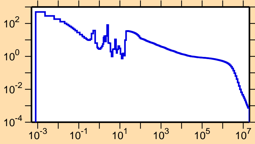
\sigma vs. E for ^{240}\text{Am}(n,\gamma)
