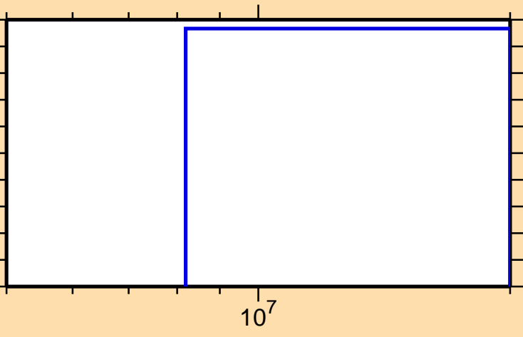
\sigma vs. E for ^{240}\text{Am}(n,2np)
