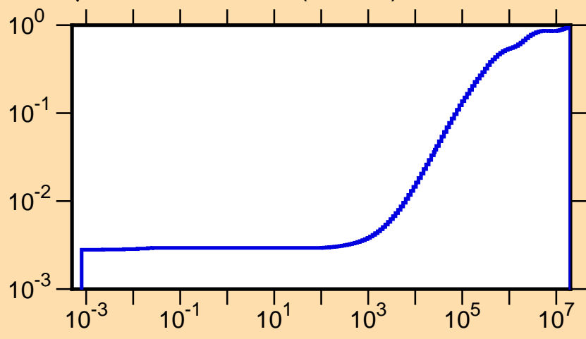
\mu vs. E for ^{241}\text{Am}(\text{mt251})
