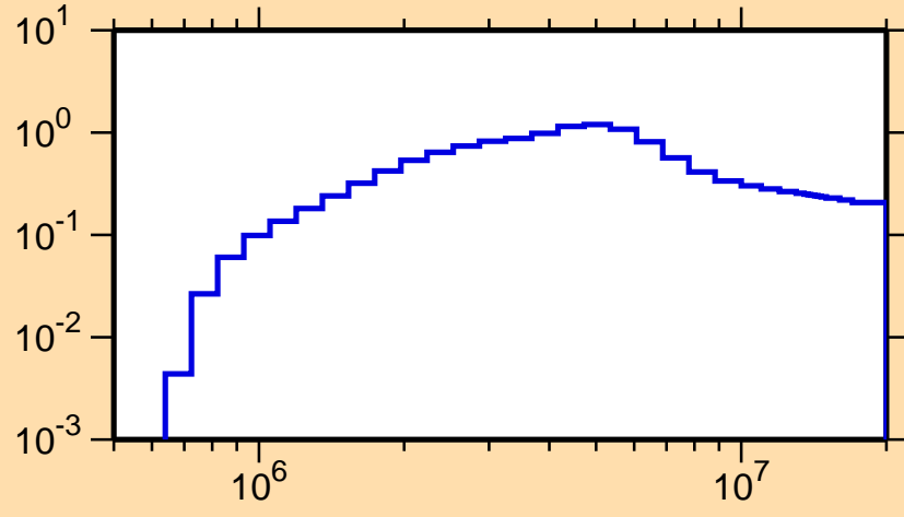
\sigma vs. E for ^{241}\text{Am}(n,n\text{cont.})
