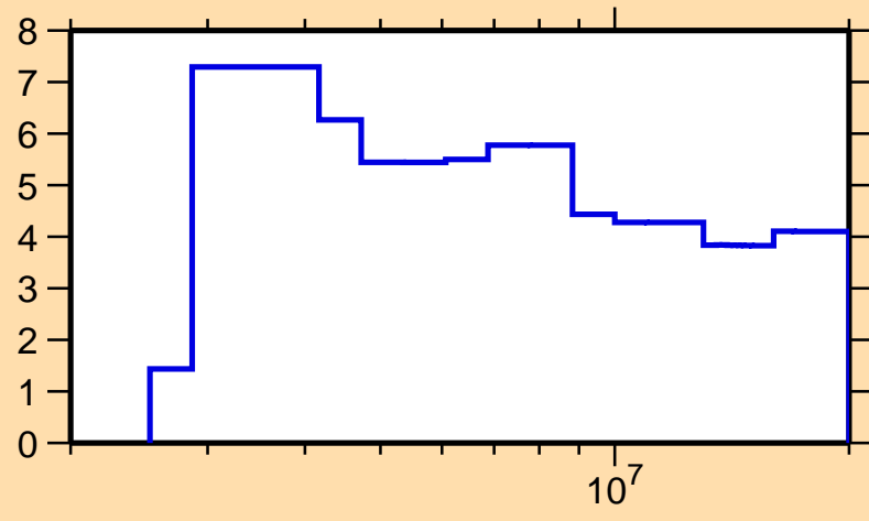
\Delta\sigma/\sigma vs. E for ^{241}\text{Am}(n,p)
