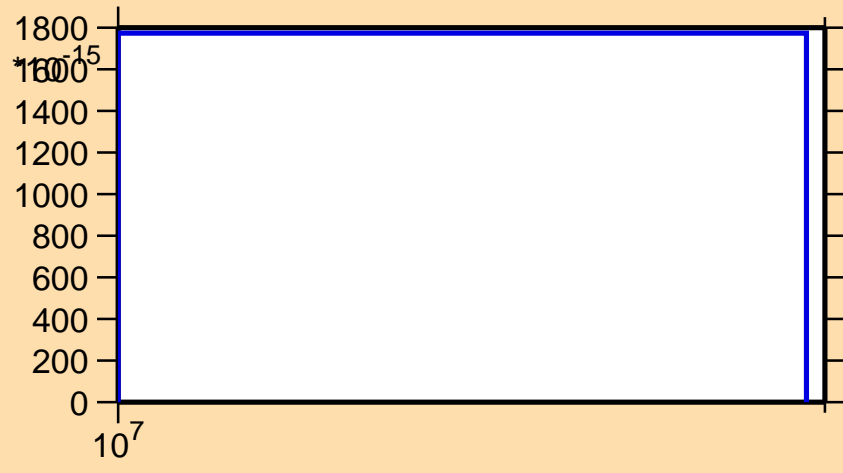
\sigma vs. E for ^{241}\text{Am}(n,\text{He}3)
