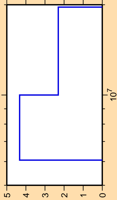
\Delta\sigma/\sigma vs. E for ^{241}\text{Am}(n,d)
