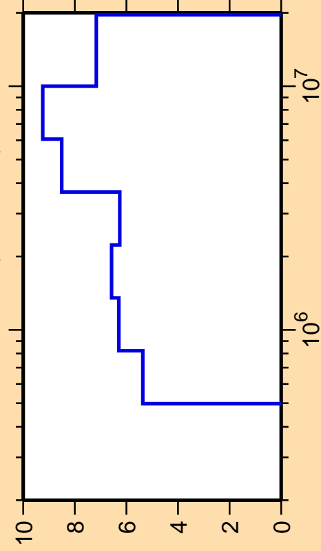
\Delta\sigma/\sigma vs. E for ^{241}\text{Am}(n,n\text{cont.})
