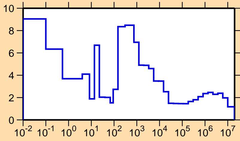
\Delta\sigma/\sigma vs. E for ^{241}\text{Am}(n,el.)
