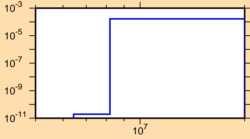
\sigma vs. E for ^{241}\text{Am}(n,d)
