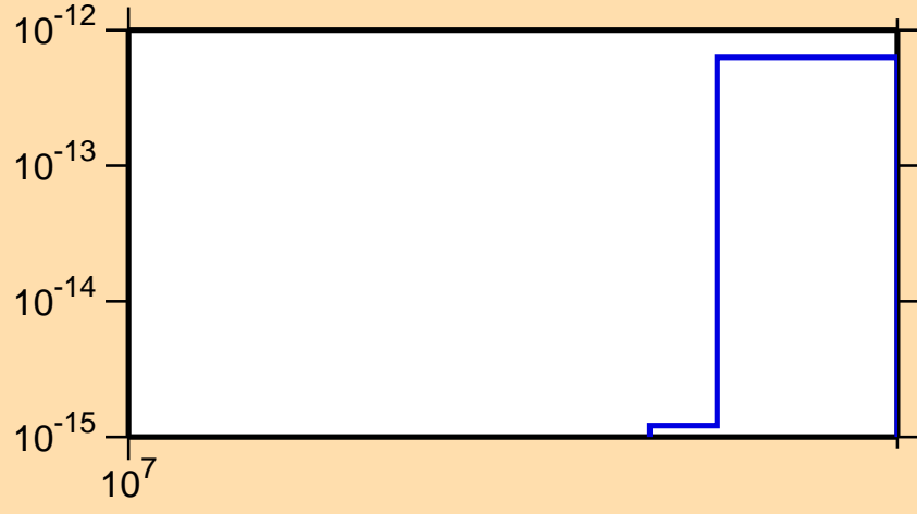
\sigma vs. E for ^{242}\text{Am} (mt 11)
