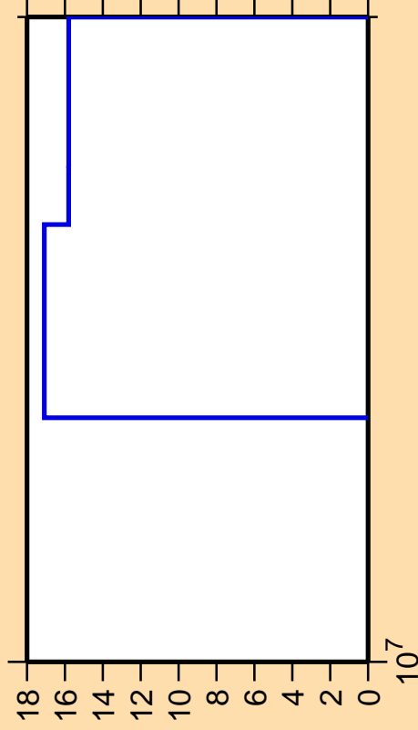
\Delta\sigma/\sigma vs. E for ^{242}\text{Am}(n,\text{nd})
