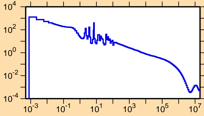
\sigma vs. E for ^{242}\text{Am}(n,\gamma)
