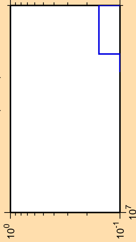
\Delta\sigma/\sigma vs. E for ^{242}\text{Am} (mt 11)
