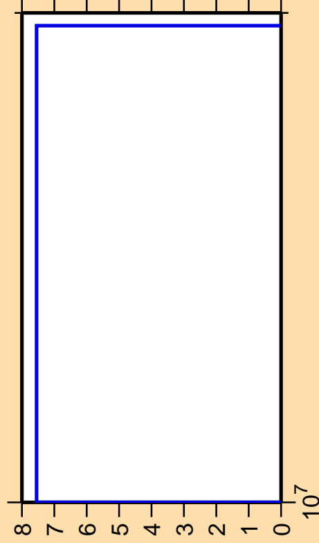
\Delta\sigma/\sigma vs. E for ^{242}\text{Am}(n,3n)
