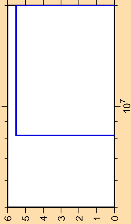
\Delta\sigma/\sigma vs. E for ^{242}\text{Am}(n,nt)
