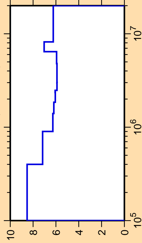
\Delta\sigma/\sigma vs. E for ^{242}\text{Am}(n,n\text{cont.})
