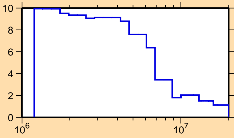
\Delta\sigma/\sigma vs. E for ^{243}\text{Am}(n, n_{\text{nonel}})
