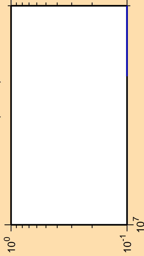
\Delta\sigma/\sigma vs. E for ^{243}\text{Am} (mt 11)
