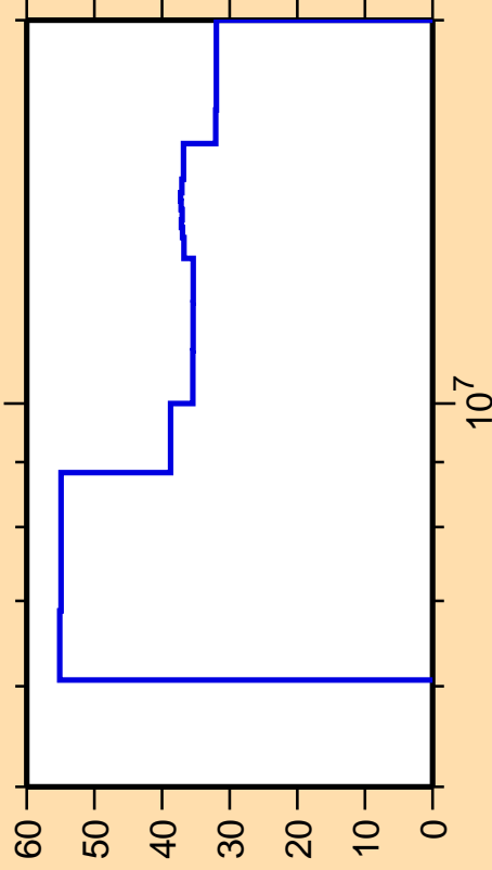
\Delta\sigma/\sigma vs. E for ^{243}\text{Am}(n,2n)
