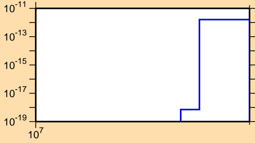
\sigma vs. E for ^{243}\text{Am} (mt 11)
