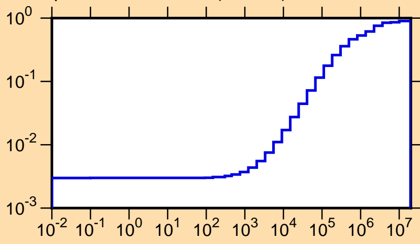
\mu vs. E for ^{243}\text{Am}(\text{mt251})
