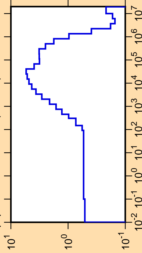
\Delta\mu/\mu vs. E for ^{243}\text{Am}(\text{mt251})
