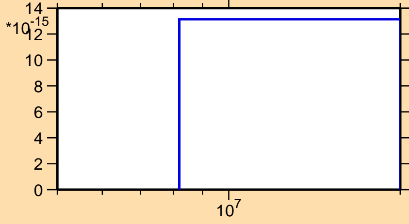
\sigma vs. E for ^{243}\text{Am}(\text{mt } 11)
