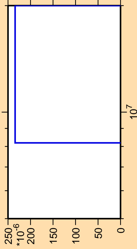
\Delta\sigma/\sigma vs. E for ^{243}\text{Am}(\text{mt } 11)
