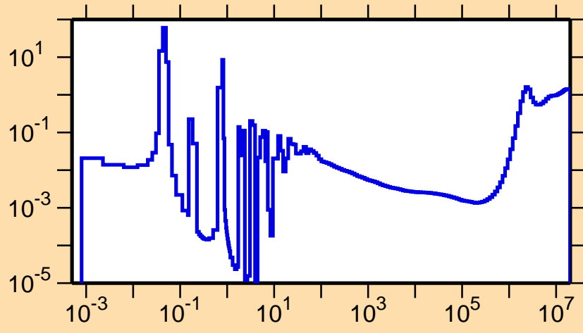
\sigma vs. E for ^{245}\text{Am}(n,f)
