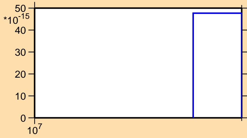
\sigma vs. E for ^{245}\text{Am} (mt 42)
