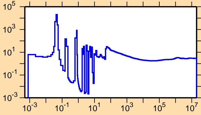
\sigma vs. E for ^{245}\text{Am}(n,\text{nonel.})
