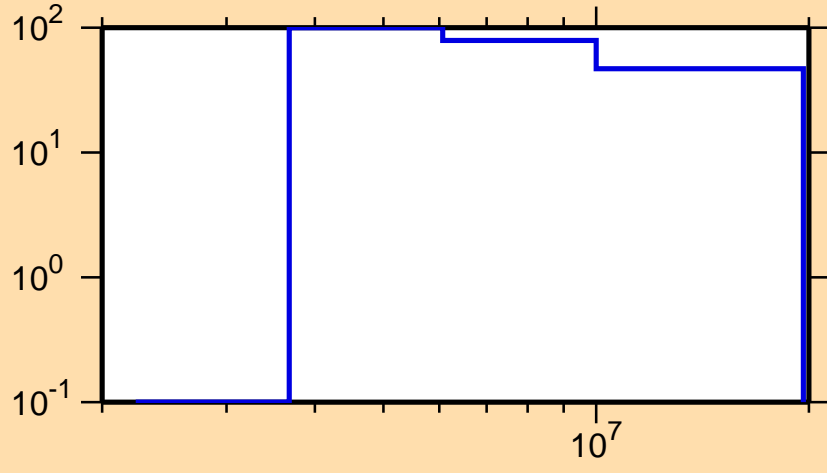
\Delta\sigma/\sigma vs. E for ^{245}\text{Am}(n,p)
