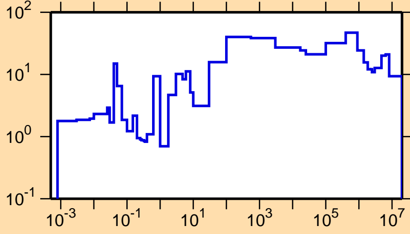
\Delta\sigma/\sigma vs. E for ^{245}\text{Am}(n,el.)
