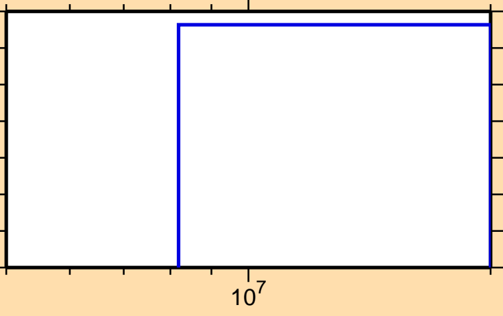
\sigma vs. E for ^{245}\text{Am}(n,3n)
