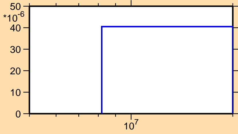
\sigma vs. E for ^{245}\text{Am}(n,t)
