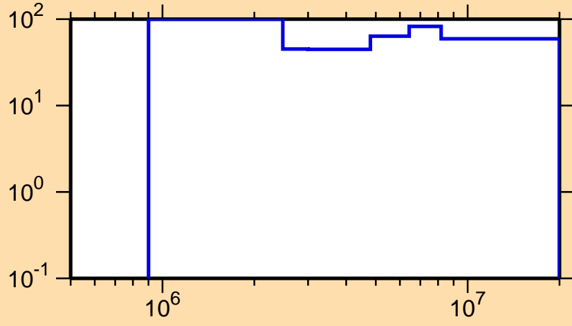
\Delta\sigma/\sigma vs. E for ^{245}\text{Am}(n,n\text{cont.})
