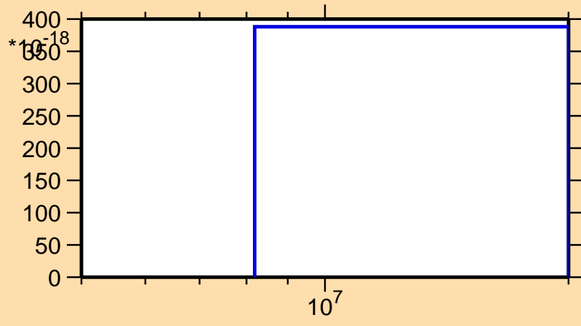
\sigma vs. E for ^{245}\text{Am} (mt 42)
