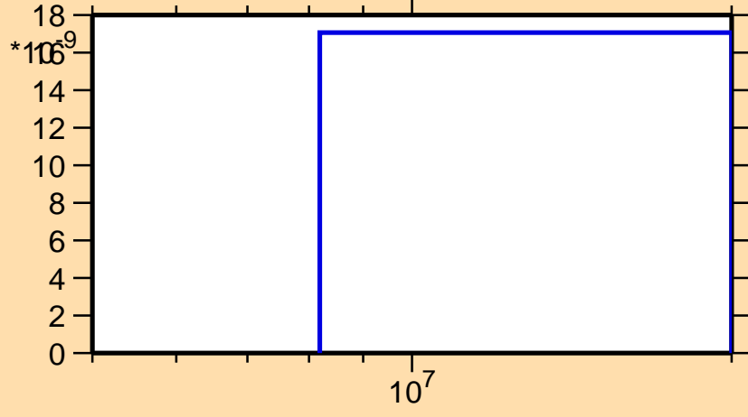
\sigma vs. E for ^{245}\text{Am}(n,\text{nd})
