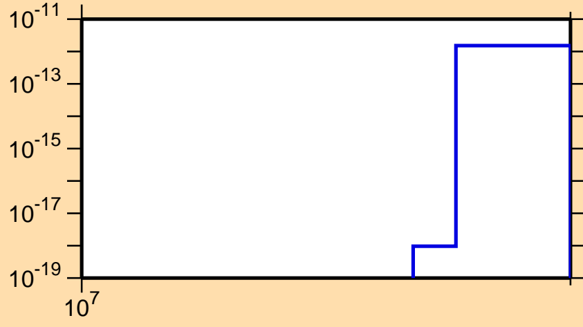
\sigma vs. E for ^{246}\text{Am} (mt 11)
